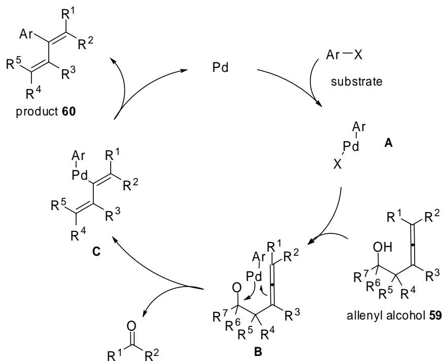
Scheme 31. Hypothesized mechanism for the achievement of 2-aryl-1,3-alkadienes.
