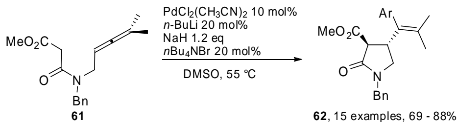
Scheme 32. Synthesis of 4-( \alpha -styryl) \gamma -lactams by \beta -aminoallene.
