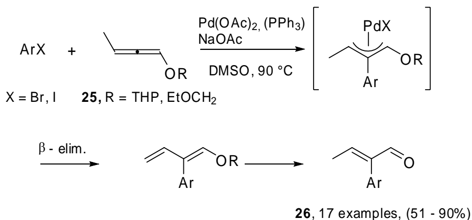
Scheme 11. Heck couplings of aryl halides and allenols to afford \alpha -arylated \alpha,\beta -unsaturated aldehydes.
