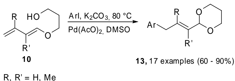
Scheme 4. Heck reaction on 1-(3-hydropropoxy)buta-1,3-dienes with aryl iodides.
