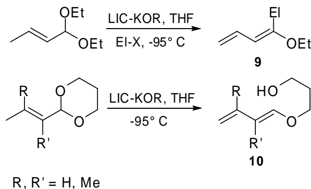
Scheme 2. Reaction of \alpha,\beta -unsaturated acetals with superbase LIC-KOR.
