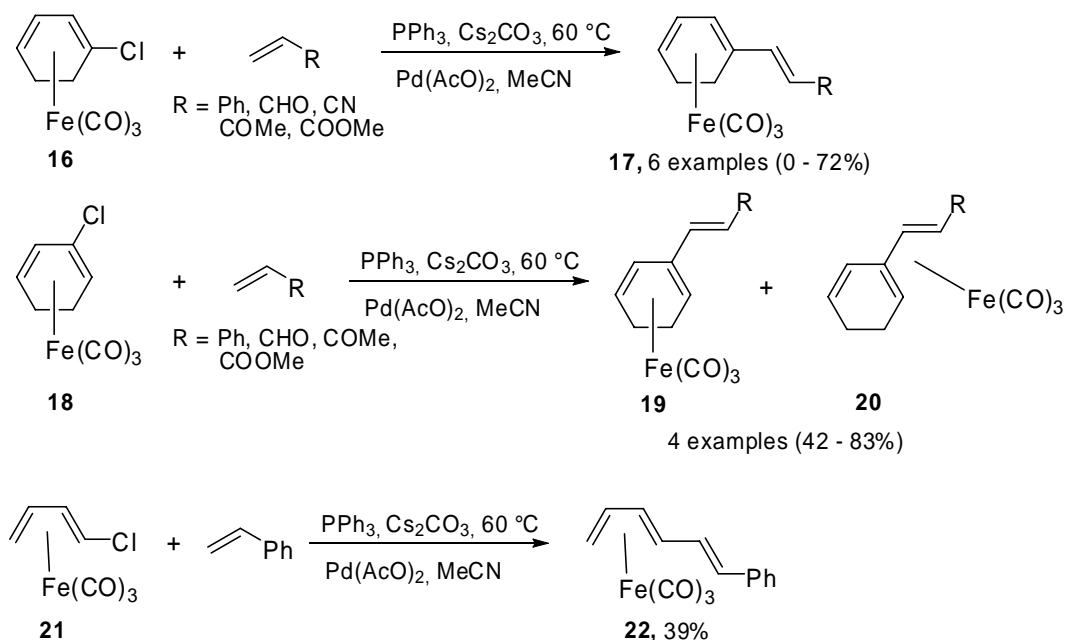
Scheme 9. Heck reactions of vinyl chlorides and diene-Fe(CO) 3 complexes.
