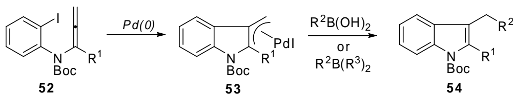
Scheme 27. Synthesis of 3-substituted and 2,3-disubstituted indoles.
