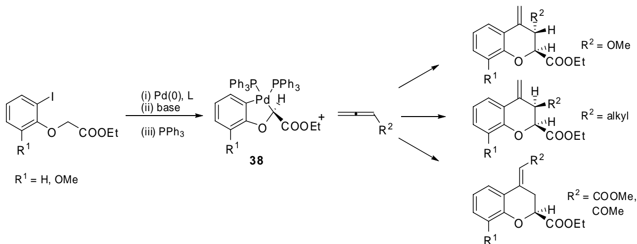
Scheme 19. Synthesis of 2,3-disubstituted 3,4-dihydro-2 H -1-benzopyrans using a polymer bounded palladicycle.
