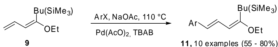
Scheme 6. Heck reaction on 1-ethoxybuta-1,3-dienes in pure TBAB.
