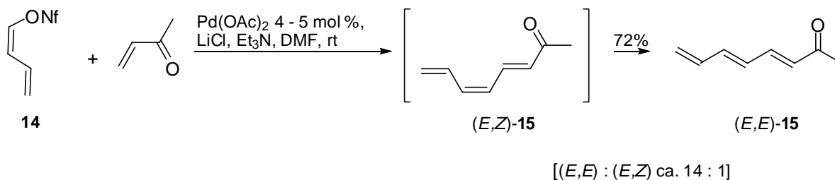
Scheme 8. Heck reaction of ( Z )-buta-1,3-dien-1-yl nonaflate.
