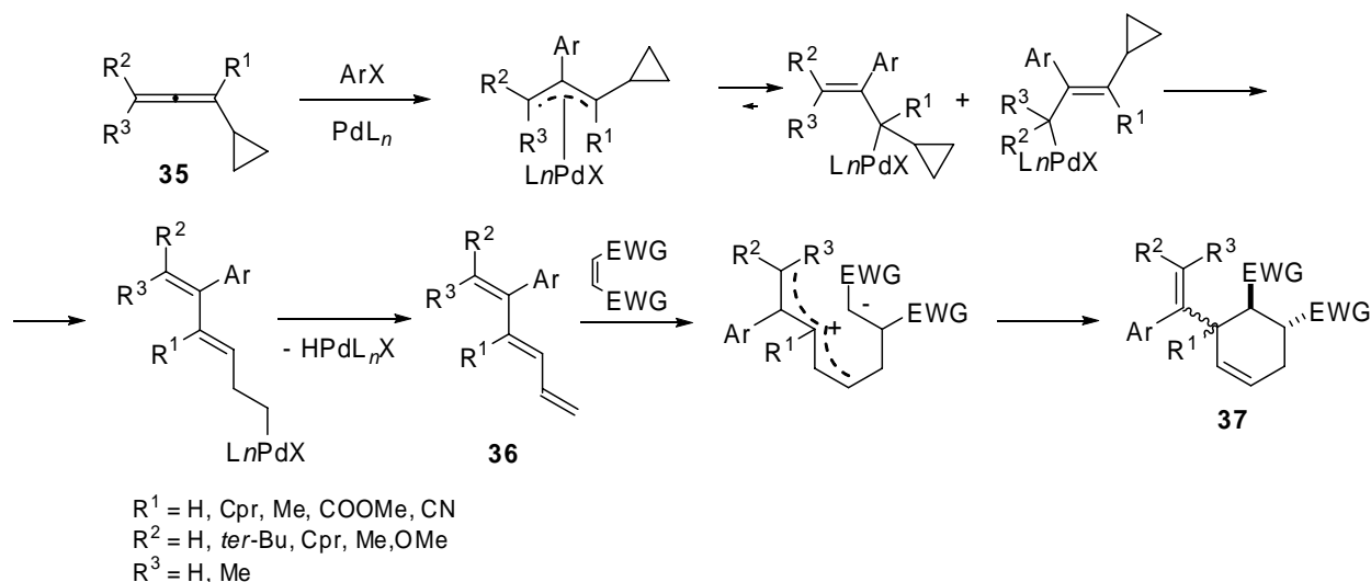
Scheme 17. Domino Heck Diels-Alder reaction by substituted 1,3-dicyclopropyl-1,2-propadienes.
