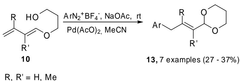
Scheme 5. Heck reaction on 1-(3-hydropropoxy)buta-1,3-dienes with arendiazonium salts.
