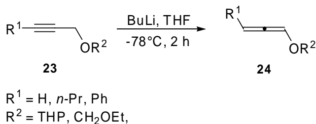
Scheme 10. Isomerization reaction of alkynes to allenes in the presence of BuLi.
