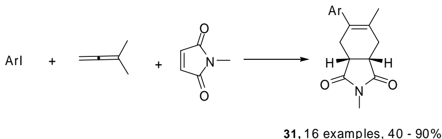
Scheme 14. Three component Heck–Diels–Alder cascade process.
