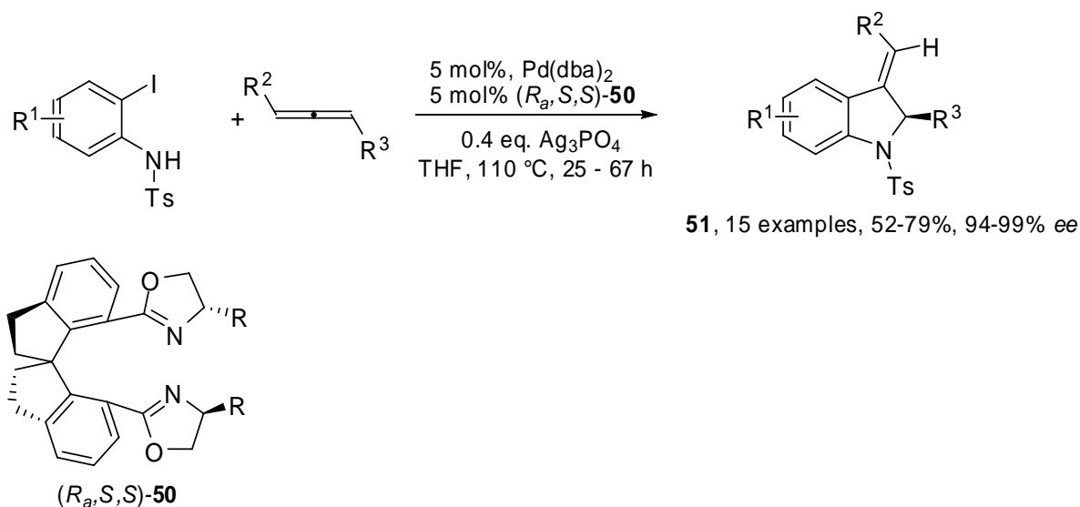
Scheme 25. Enantioselective heteroannulations between allenes and 2-iodoanilines.
