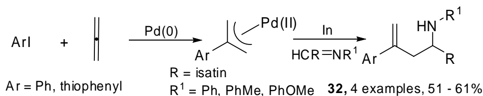
Scheme 15. Cascade allylation of isatin imines.
