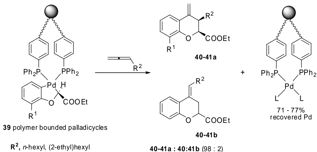
Scheme 20. Annulation reaction of heteroatom-substituted allenes.
