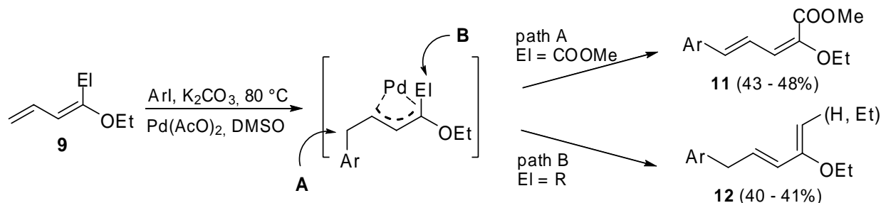
Scheme 3. Heck reaction on 1-ethoxy-buta-1,3-dienes.
