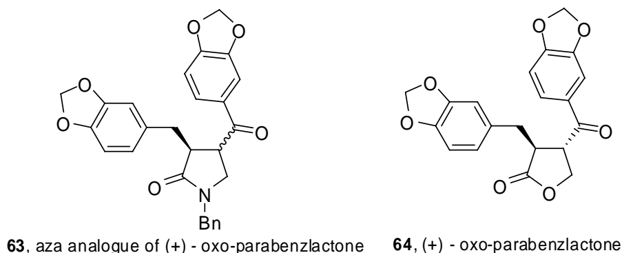
Figure 1. Aza analogue of oxo-parabenzlactone.
