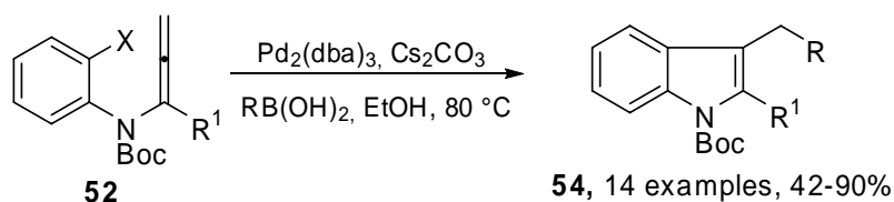
Scheme 27. Synthesis of 3-substituted and 2,3-disubstituted indoles.
