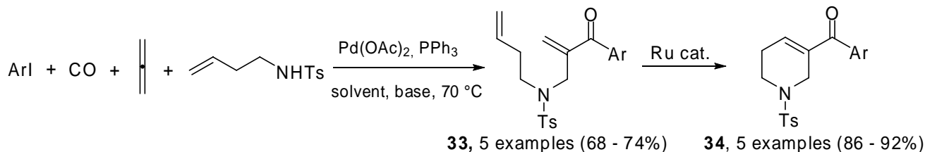
Scheme 16. Four-component Pd(0) catalyzed cascade/ring closing metathesis.
