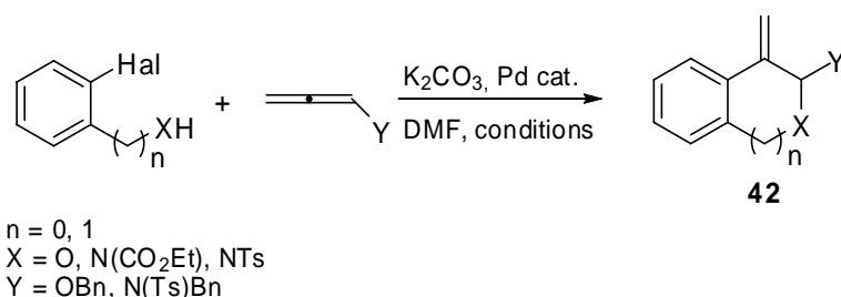
Scheme 20. Annulation reaction of heteroatom-substituted allenes.
