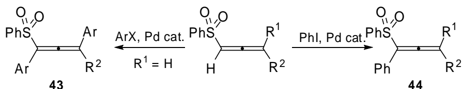
Scheme 21. Heck type allenylation of aryl halides with allenes.
