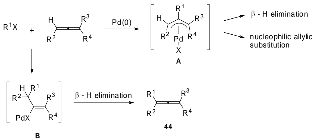
Scheme 22. Proposed mechanism for the carbopalladation of allenes.
