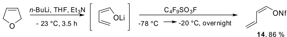
Scheme 7. Synthesis of ( Z )-buta-1,3-dien-1-yl nonaflate by lithiation of 2,5-dihydrofuran.
