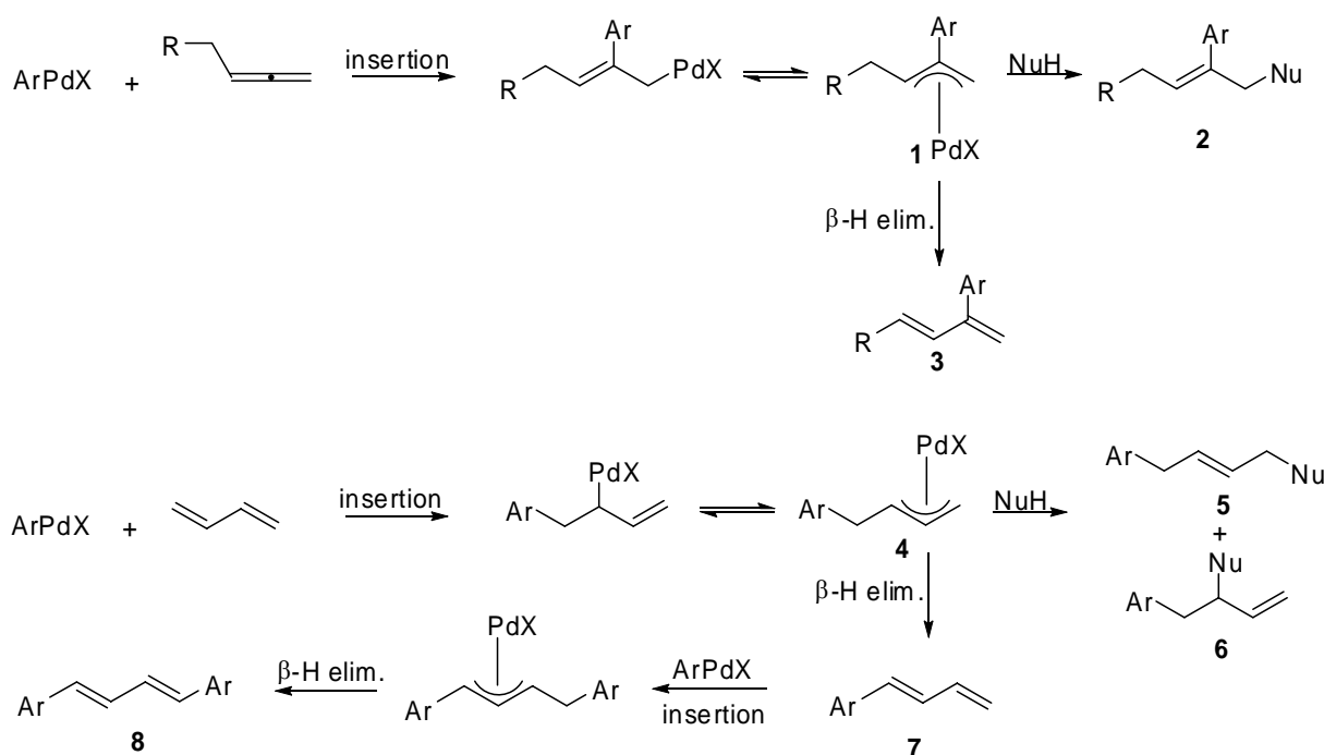
Scheme 1. General reactivity of 1,2- and 1,3-dienes in Mizoroki–Heck reaction.
