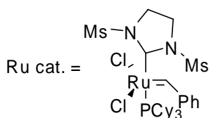
Scheme 17. Domino Heck Diels-Alder reaction by substituted 1,3-dicyclopropyl-1,2-propadienes.
