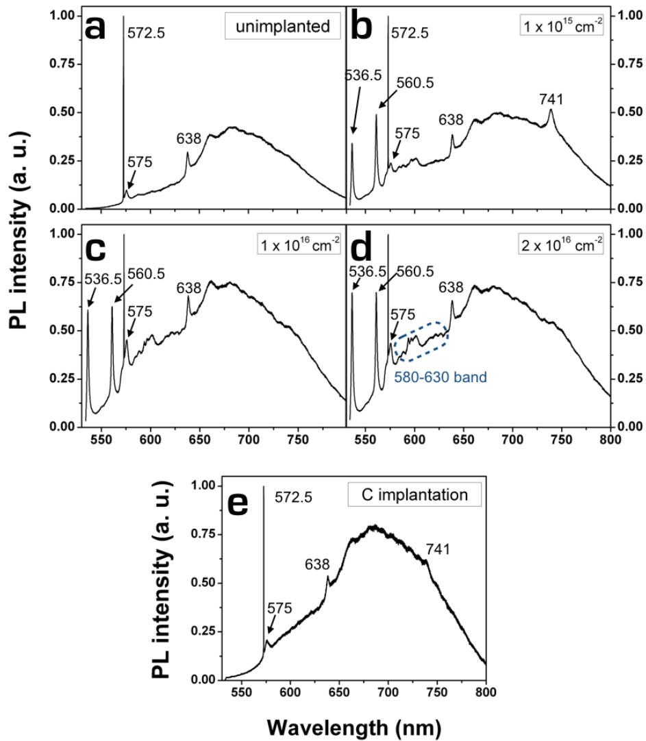
Figure 1: PL spectra acquired at 532 nm excitation from He-irradiated “optical grade” diamond substrates: a) control unirradiated region (sample #1); b) 1 MeV He + irradiation, 1 \times 10^{15} \text{ cm}^{-2} fluence (sample #2); c) 1.3 MeV He + irradiation, 1 \times 10^{16} \text{ cm}^{-2} fluence (sample #1); d) 1.3 MeV He + irradiation, 2 \times 10^{16} \text{ cm}^{-2} fluence (sample #1); e) sample #3 irradiated with a 6 MeV C + beam at 2 \times 10^{15} \text{ cm}^{-2} fluence.
