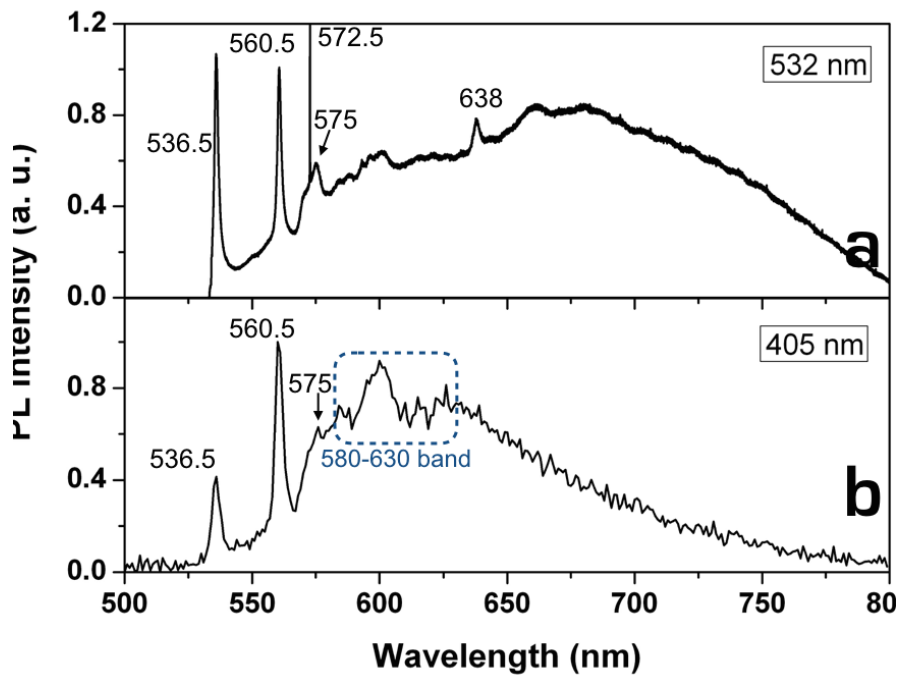
Figure 4: PL spectra acquired under different excitation wavelengths from sample #1, upon the 1.3 MeV He + irradiation at 1 \times 10^{16} cm -2 fluence and subsequent thermal annealing: a) 532 nm excitation; b) 405 nm excitation.
