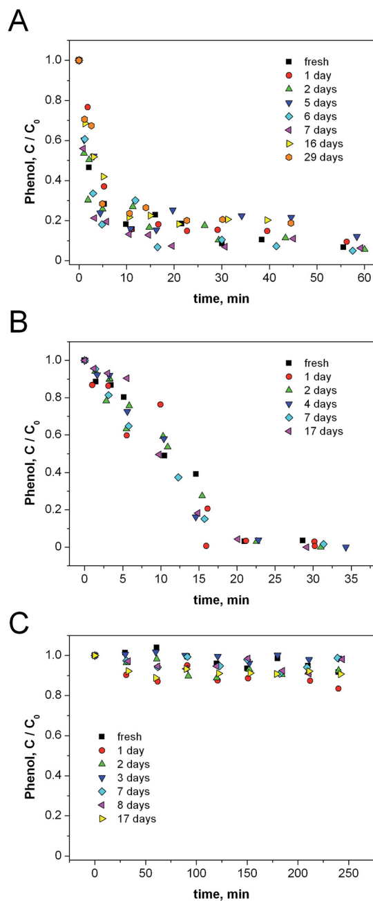
Fig. 6 Time trend of phenol (initial concentration 0.1 mM) in the presence of 1 mM \text{H}_2\text{O}_2 and 0.1 g \text{L}^{-1} pZVI. The pZVI stock aqueous suspension (1 g \text{L}^{-1} loading) was stored in the presence of air for the reported amount of time prior to use. (A) pH 2; (B) pH 4; (C) pH 6. The pH values were adjusted by addition of \text{HClO}_4 .
