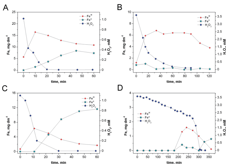
Fig. 5 Time trends of \text{Fe}^{\text{III}} , \text{Fe}^{\text{II}} (left Y-axis) and \text{H}_2\text{O}_2 (right Y-axis), in the presence of 0.1 mM phenol, 0.1 \text{ g L}^{-1} pZVI, and: (A) 1 mM \text{H}_2\text{O}_2 at pH 2; (B) 3.5 mM \text{H}_2\text{O}_2 at pH 2; (C) 1 mM \text{H}_2\text{O}_2 at pH 3; (D) 3.5 mM \text{H}_2\text{O}_2 at pH 3. The pH values were adjusted by addition of \text{HClO}_4 .
