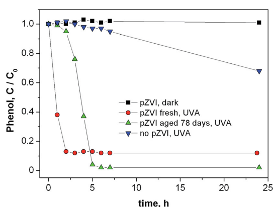
Fig. 7 Time trend of phenol (initial concentration 0.1 mM) in the presence of 1 mM \text{H}_2\text{O}_2 and, according to the different experiments (see figure legend): (■) fresh pZVI (0.1 g \text{L}^{-1} ) in the dark ("fresh pZVI" denotes the material that underwent initial ageing in air but did not undergo additional ageing in aqueous suspension); (●) fresh pZVI (0.1 g \text{L}^{-1} ) under UVA irradiation; (▲) aged pZVI (0.1 g \text{L}^{-1} ) under UVA irradiation (this material was aged in aqueous suspension for 78 days), and (▼) no pZVI under UVA irradiation. In all the experiments the pH value was 5, adjusted with \text{HClO}_4 .
