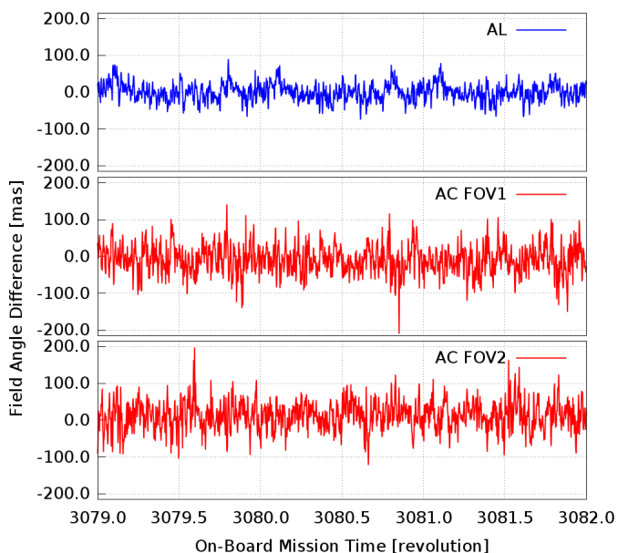
Fig. 3. Comparison of the first and second on-ground attitudes for the \eta , \zeta_1 and \zeta_2 field angles (AL and AC) for 18 hours of mission data, where the indices 1 and 2 refer to the two Gaia telescopes (i.e. fields of view).
