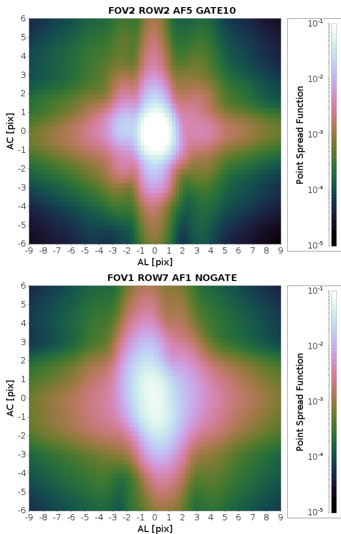
Fig. 10. Examples of the PSF for the devices with the smallest (93.1 mas) and largest (132.4 mas) AL FWHMs. The largest FWHMs are in devices in one corner of the focal plane (AF1/2 in rows 6 & 7), while the smallest FWHM is close to the centre (AF5, row 2). The longer gates usually have larger FWHMs in the AL profile due to the variation in the PSF along the CCD. We also see here the effect of the greater AC smearing in the ungated PSF profile.
