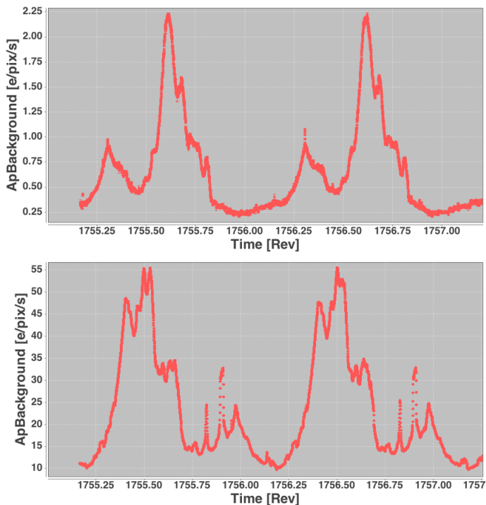
Fig. 6. (top) Example large-scale background model in the centre of BP device on row 1 over a period of two spacecraft revolutions in early January 2015; (bottom) the same for AF4 on row 7. The former exhibits background levels and variations amongst the lowest over the astro/photo focal plane, while the latter exhibits the largest.
