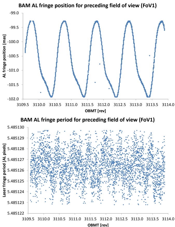
Fig. 19. BAM daily First-Look analysis. The BAM data quality is monitored on a daily basis using several metrics implemented in the First-Look system. The top panel shows the evolution of the fringe phase for the preceding field of view during four spacecraft revolutions beginning on 2015-12-15. The significant ( \approx 1 mas) amplitude of the periodic variations is apparent. The bottom panel shows the evolution of a secondary (nuisance) parameter, namely the average fringe period, during the same interval ( \approx 1 ppm variability in this case). The plots include average values computed by First Look but have been adapted for better visualisation.
