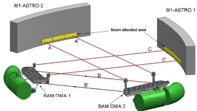
Fig. 17. BAM overview. The BAM is a laser interferometer that injects two beams in each telescope entrance pupil. In this way, an interference pattern is produced for each telescope in the common focal plane. The relative shift of the patterns at the CCD level is related to changes in the basic angle between the telescopes. Credit: Airbus Defence & Space.
