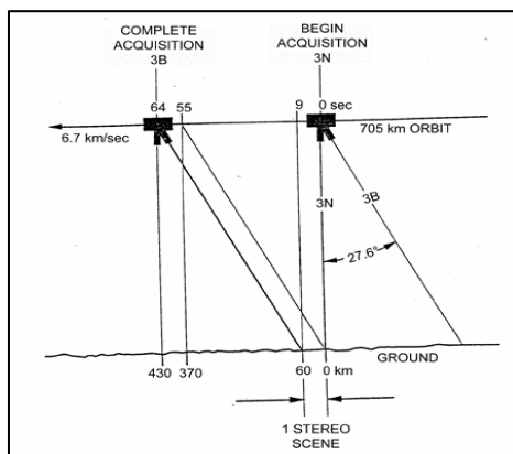
Fig. 2. ASTER stereo pairs recording sheme (HAROLD R. LANG, ATBD- AST-08 document).
