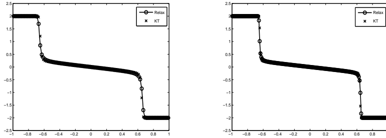
Fig. 1. Non-convex flux. Kurganov-Tadmor and relaxation schemes, with n = 100 (left) and n = 200 (right).
