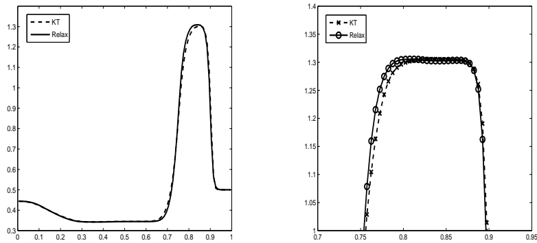
Fig. 2. Lax Riemann problem, density component. KT (dashed) and relaxation (solid line) with n = 100 (left) and n = 200 (right), where a detail of the density peak is shown.
