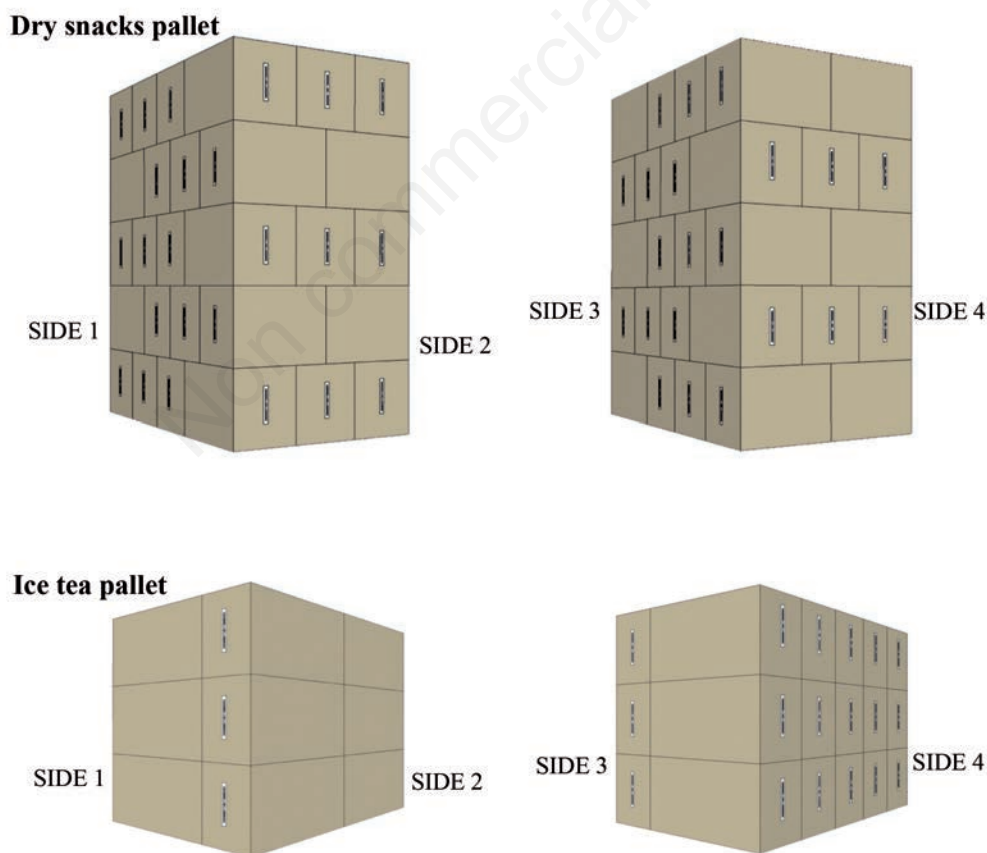
Figure 1. Dry snack and ice tea pallets setup. On the pallets are superimposed 45 or 21 carton boxes respectively. Each carton box is electronically identified by means of an ultra high frequency radio frequency identification transponder (UH331 LabID) applied on the carton box minor side, in external position.
