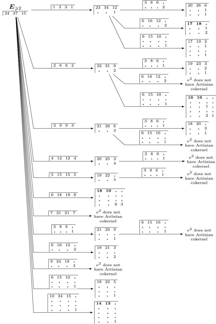
FIGURE 1. The set of constant rank matrices that can be produced with our method applied to the truncation E_{\geq 2} = \bigoplus_{t \geq 2} H^0(\mathbb{P}^2(t-1)) the module of global sections of a twist of the tangent bundle E = T_{\mathbb{P}^2}(-1) .
