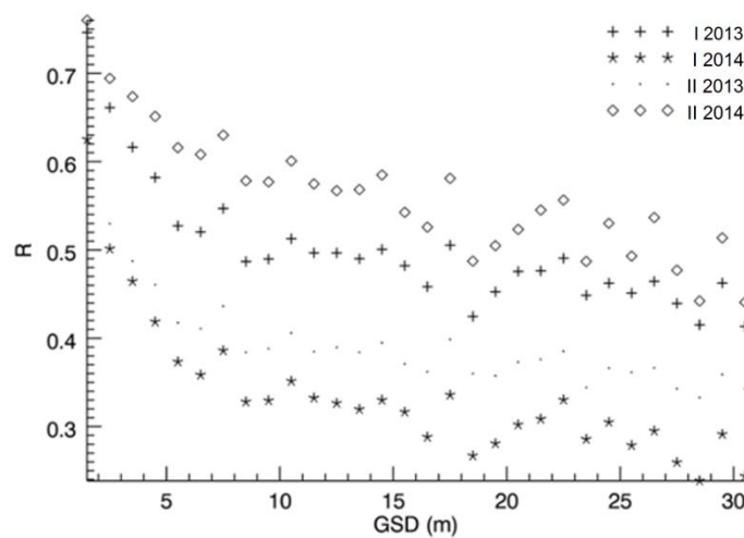
20 Fig. 5 R_1 vs GSD. The role of GSD in conditioning consistency between images acquired at different spatial resolutions; trends refer 21 to the four acquisition dates ("I" and "II" like in Table 3).
