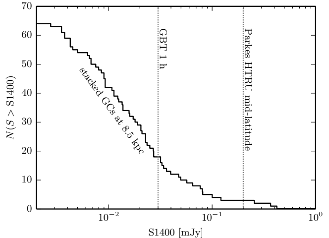
Figure 1. Complementary cumulative distribution of flux densities at 1.4 GHz, S1400, of the 64 pulsars in the globular clusters that are listed in Tab. 1, rescaled to a distance of 8.5 kpc. We show for comparison the limiting flux density, \sim 0.2 mJy, of the Parkes High Time Resolution Universe (HTRU) mid-latitude survey (Keith et al. 2010) as well as the reference GBT survey, 0.03 mJy (discussed in Sec. 3). The plot illustrates that a survey that is significantly deeper than that with Parkes would start probing the radio luminosity function in a regime that is well supported by data. Predictions for radio-bright bulge MSPs ( S1400 \geq 10 \mu\text{Jy} ) are built upon 43 measured globular cluster MSPs.
