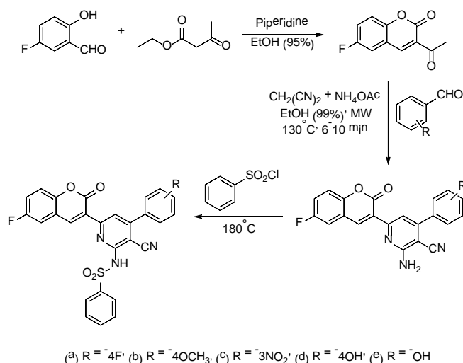
Scheme 14. Synthetic pathway.
