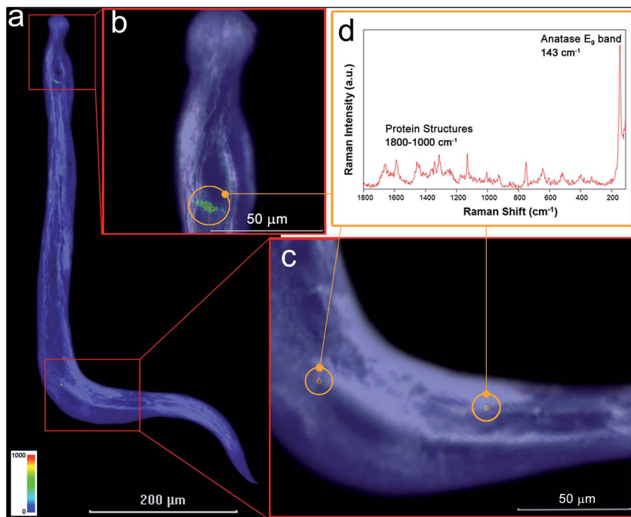
Fig. 3 Raman mapping on C. elegans fed with 0.2 \text{ mg ml}^{-1} commercial Sigma \text{TiO}_2 NPs for 24 h. Contrast phase image of the worm overlaid with a Raman map obtained from monitoring the E_g band intensity at 143 \text{ cm}^{-1} over the area analyzed. A color scale from blue to red was used to visualize the intensity of the anatase E_g band (a). Orange circles show the magnification of the pharyngeal (b) and vulval (c) regions of the worm, showing \text{TiO}_2 NPs agglomerates. Raman spectrum collected on \text{TiO}_2 NPs agglomerate shows the anatase E_g band at 143 \text{ cm}^{-1} and protein structures of worm tissues in the range 1800\text{--}1000 \text{ cm}^{-1} (d).
