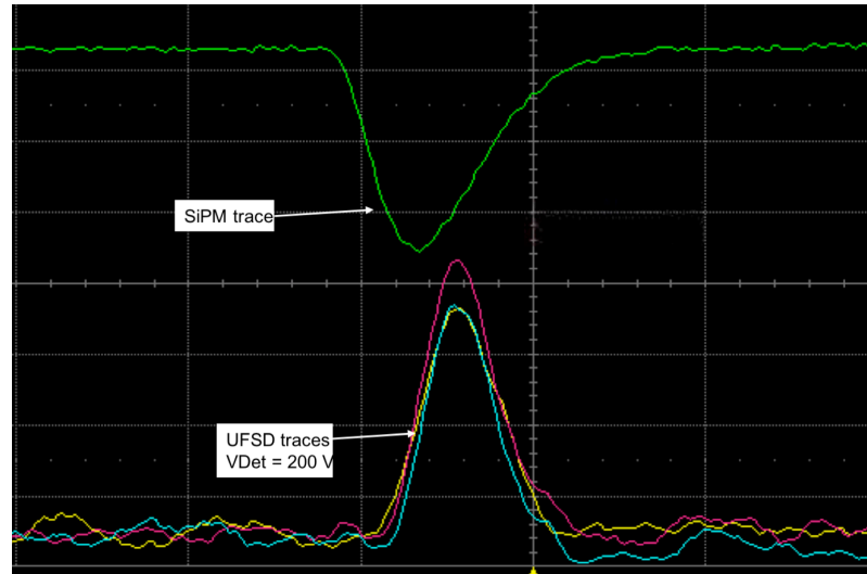
Figure 5 Screenshot of one event, showing the signals of 3 UFSD biased at 200 V and the SiPM at 28 V. Each horizontal division corresponds to 2 ns, while each vertical division is 100 mV.
