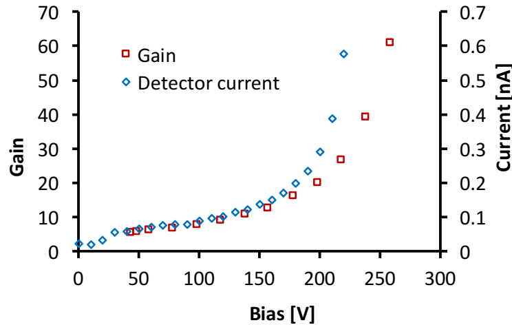
Figure 1 Bias dependence of the leakage current and the signal gain for a 45 \mu\text{m} -thick UFSD sensor with an area of 1.7 \text{ mm}^2 . The gain determination is subject to an overall scale uncertainty of 20%. The similar exponential behaviour of gain and sensor current below 200 \text{ V} bias is due to the common charge multiplication mechanism.
