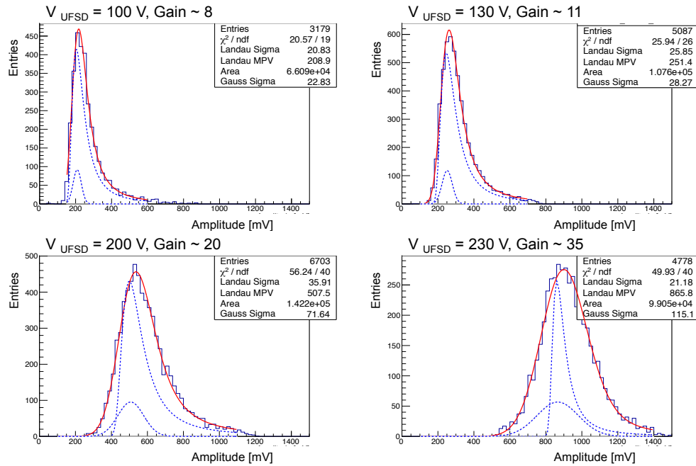
Figure 6 Distribution of the signal amplitude at four values of the detector Vbias: (100V,130V , 200V and 230V), with superposed the curves from a Landau-Gauss convolution fit (solid red curve). On each graph, the normalizations of the Landau and Gauss components are arbitrary as only their product is defined. Likewise, for explanation purposes only, the gaussian curve is arbitrarily aligned with the Landau MPV value.
