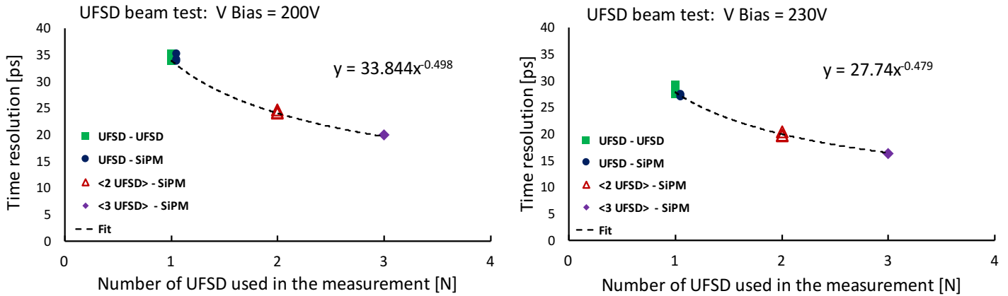
Figure 8 Timing resolution for: single UFSD (N=1) obtained from the UFSD-SiPM and UFSD-UFSD time differences; averaged pairs of UFSD (N=2) and average of 3 UFSD (N = 3) for bias voltages of (left) 200V and (right) 230V.
