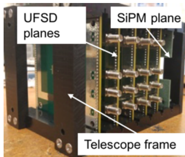
Figure 4 Beam Test frame showing four UFSD boards and the trigger counter. Alignment was assured with four rods (not shown) going through aligning holes in the four corners of the boards and the frame.
