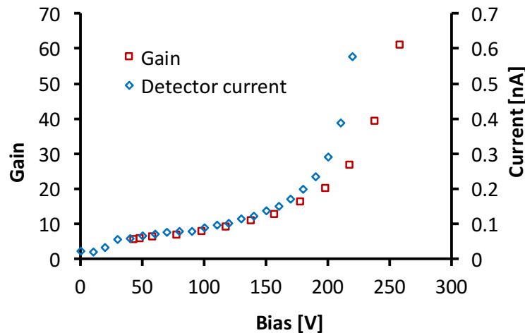
Figure 1 Bias dependence of the leakage current and the signal gain for a 45 \mu\text{m} -thick UFSD sensor with an area of 1.7 \text{mm}^2 . The gain determination is subject to an overall scale uncertainty of 20%. The similar exponential behaviour of gain and sensor current below 200 \text{V} bias is due to the common charge multiplication mechanism.
