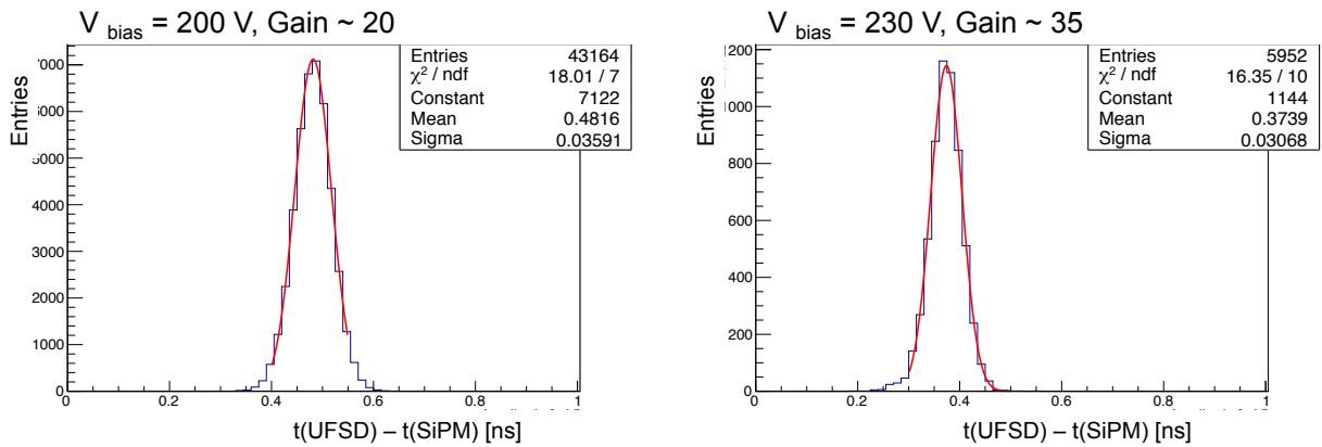
Figure 7 Time difference UFSD-SiPM at 2 different UFSD bias voltages: 200 V with sigma = 36 ps, and 230 V with sigma = 31 ps.
