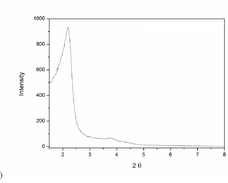
Figure S3. Small angle XRD of AuPt/MCM-41 a) before and b) after reaction.
