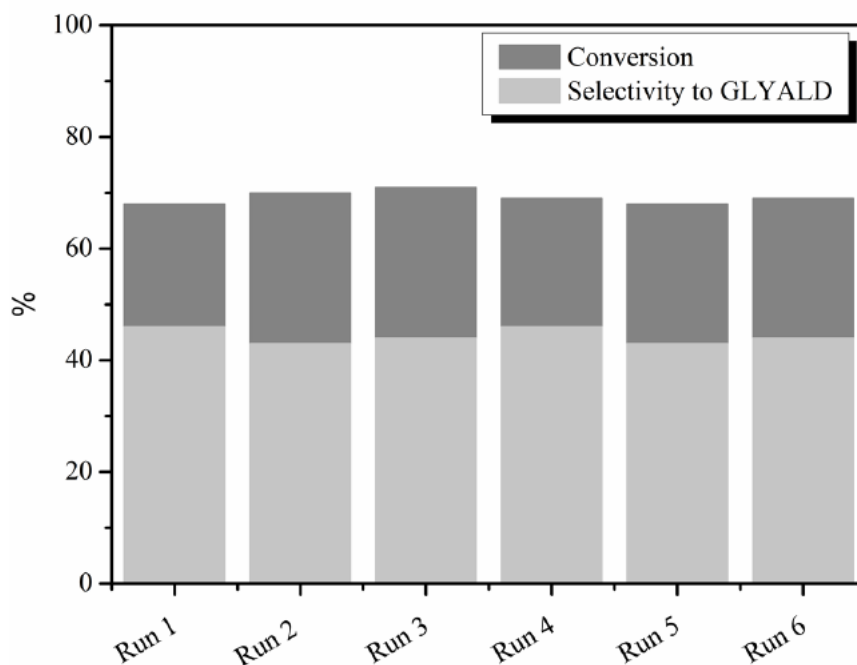
Figure S2. Recycling tests using AuPt/MCM41. Glycerol 0.3M in water; metal/alcohol = 1/500 mol/mol; 300kPa O 2 ; T=80°C.
