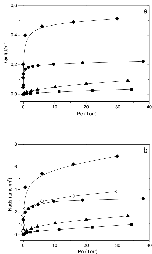
Fig.3 Section a: surface area-normalized calorimetric isotherms (integral heats vs. equilibrium pressure). Section b, surface area-normalized volumetric isotherms ( \mu\text{molNH}_3 adsorbed vs. equilibrium pressure). (-■-) AuPt/MCM41; (-▲-) AuPt/SiO 2 ; (-●-) AuPt/H-Mord; (-◆-) AuPt/S-ZrO 2 ; (-◇-) AuPt/S-ZrO 2 without Lewis sites contribution.
