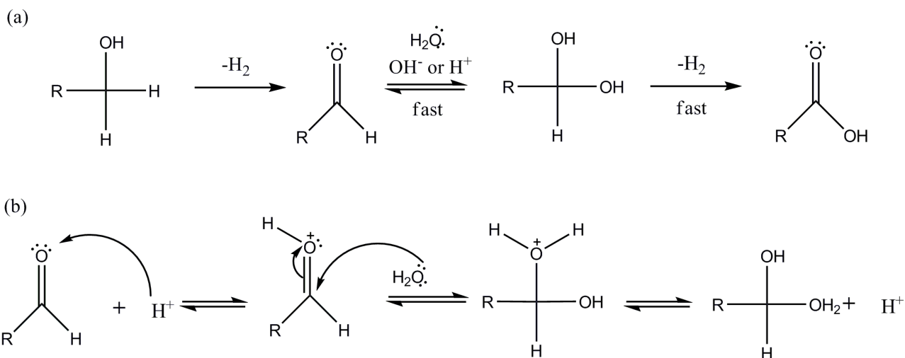
Scheme 2 a) Alcohol dehydrogenation mechanism in the presence of water and b) acid catalyzed geminal diol formation.
