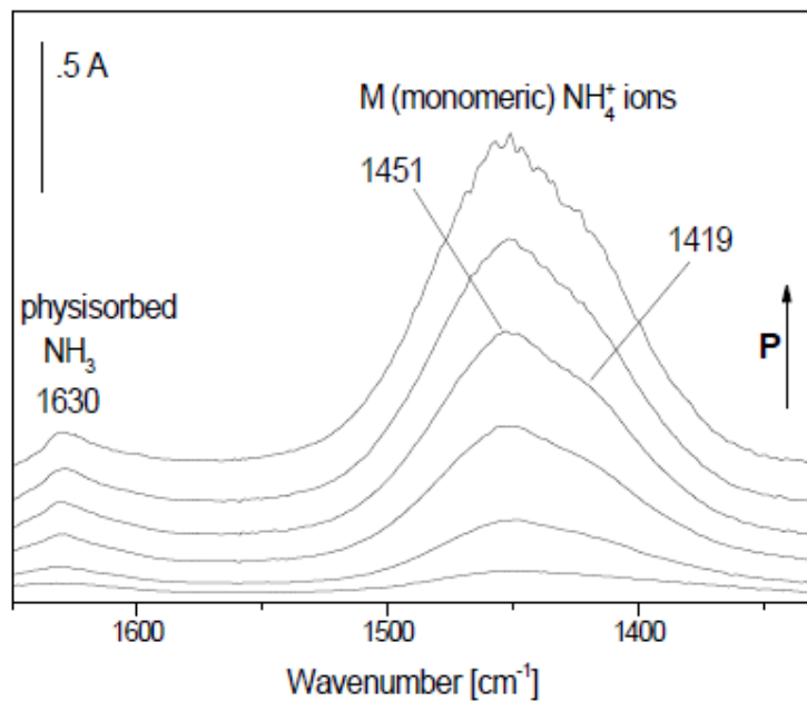
Figure S8. FTIR spectra of \text{NH}_3 adsorbed at 373 K on AuPt/H-Mordenite.
