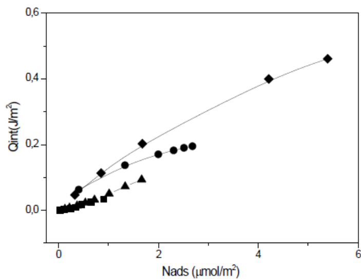
Figure S9. Q_{\text{int}} as function of the \mu\text{mol} of adsorbed \text{NH}_3 : (-■-) AuPt/MCM41; (-□-) AuPt/SiO 2 ; (-□-) AuPt/H-Mord; (-□-) AuPt/S-ZrO 2 ;
