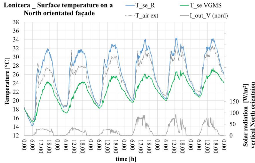
Fig. 19. Demonstration building with Lonicera nitida . Comparison of the external surface temperature between the reference wall ( T_{se\_R} ) and the VGMS wall ( T_{se\_VGMS} ) both of which are north oriented.
