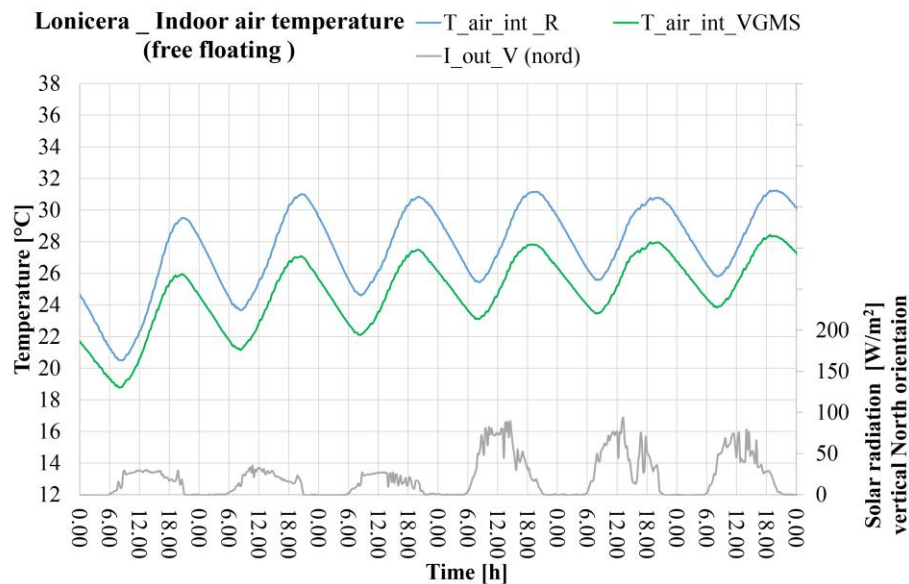
Fig. 20. Demonstration building, with Lonicera nitida . Comparison of the indoor air temperature between the room with the reference technology (wooden cladding T_{air\_int\_R} ) and the room with the VGMS ( T_{air\_int\_VGMS} ). Measurements conducted in free floating conditions.
