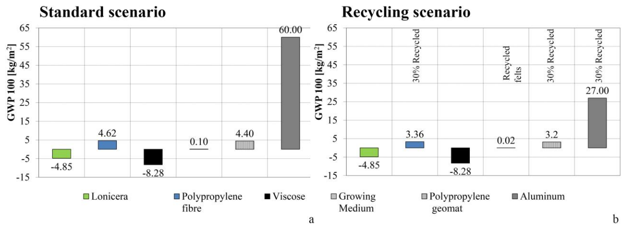
Fig. 8. a) GRE_EN_S Global Warming Potential (target of 100 years) for the reference scenario. b) GRE_EN_S Global Warming Potential (target of 100 years) for the recycling scenario.
