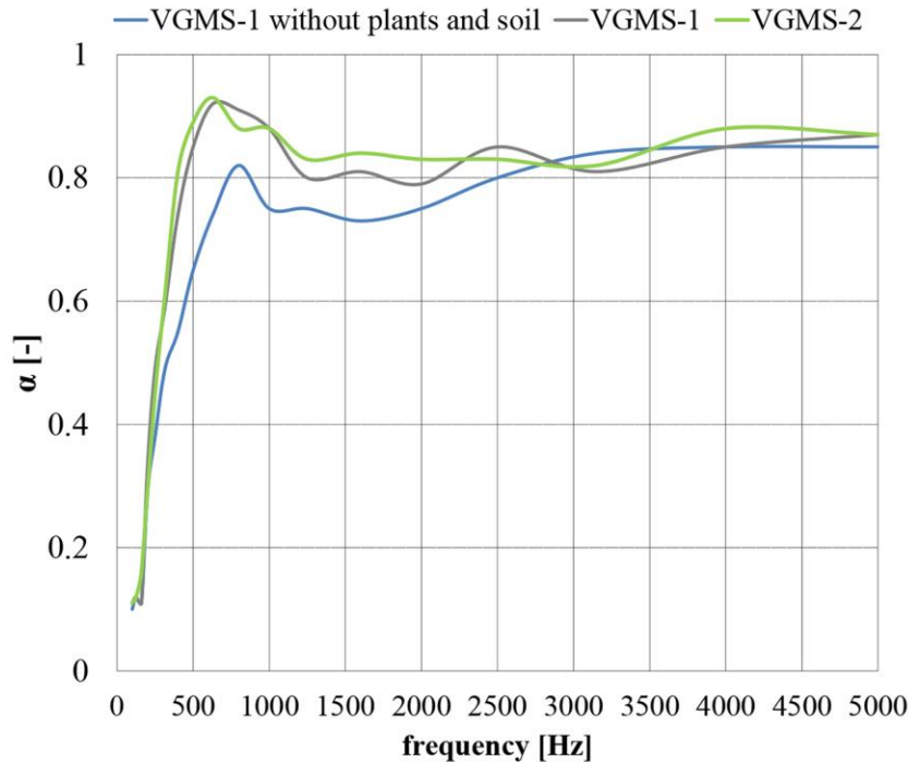
Fig. 15. Experimental sound absorption coefficient results in the reverberation room. The three different prototypes measured in the reverberation room were: VGMS_1, VGMS_1 without plants and soil, VGMS_2 (c).
