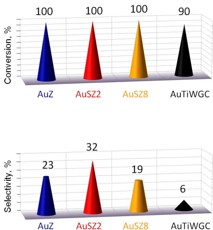
Figure 5: Catalytic performances for the oxidative esterification of HMF to FDMC. (reaction at 130 °C - 3 bar O 2 - 5 h of reaction).
