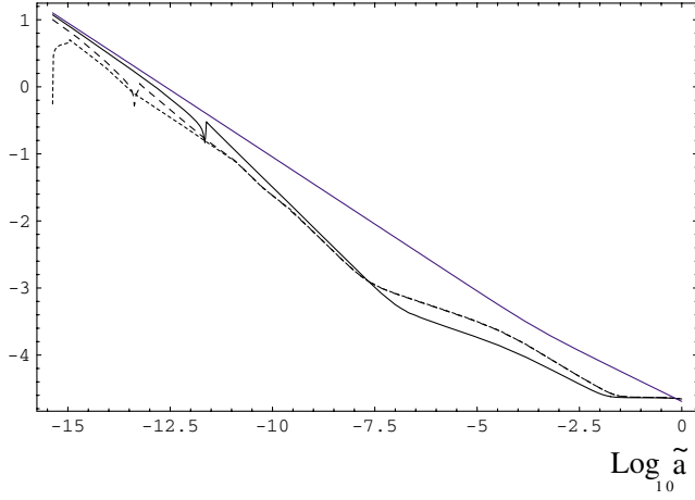
FIG. 2 (color online). Evolution of the energy density of the background (upper solid line) and of three typical solutions for the scalar field. We see that different initial conditions converge to the same solution.
