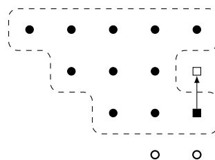
(a) The Borel set \{I_4\} defined by I = (x_2^2, x_2 x_1, x_1^3) .
