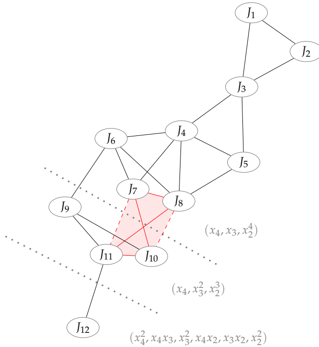
Figure 3.12: The Borel incidence graph of \mathbf{Hilb}_{4t+1}^4 . The light red quadrangle corresponds to the family over \mathbb{P}^1 \times \mathbb{P}^1 and the dashed lines correspond to composed Borel rational deformations. The dotted lines divide the ideals w.r.t. the hyperplane section.
