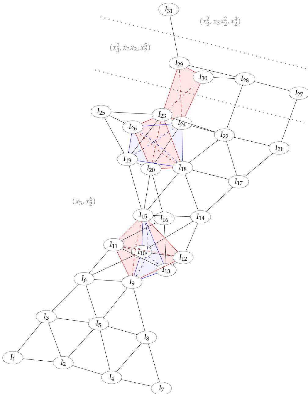
Figure 3.14: The Borel incidence graph of \mathbf{Hilb}_{6t-3}^3 .
