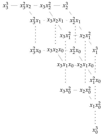
Figure 2.8: The Marinari’s lattice describing the poset \mathcal{P}(3, 3) (cf. Figure 2.3).
