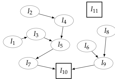
(h) The DegRevLex-deformation graph of \mathbf{Hilb}_{6t-5}^3 .
