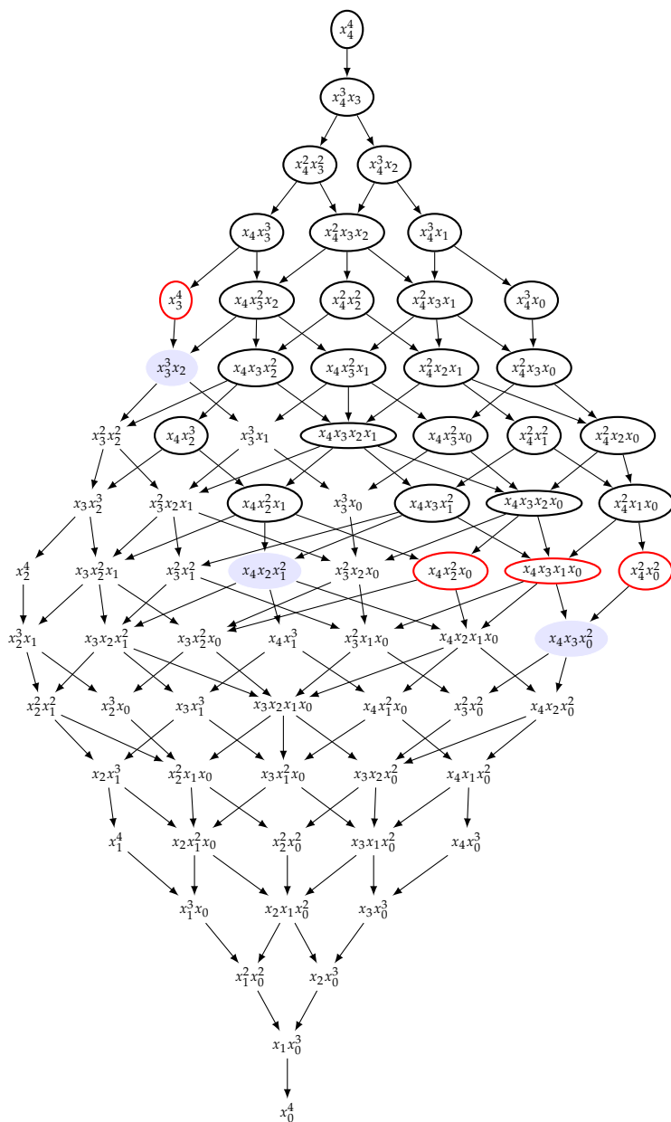
Figure 2.13: The Borel set defined by the ideal (x_4^2, x_4x_3^2, x_4x_3x_2, x_4x_2^2, x_4x_3x_1, x_3^4) in \mathcal{P}(4,4) . The monomials with red boundary are minimal elements of the Borel set, whereas the monomials with a light blue background are maximal elements in the complement.
