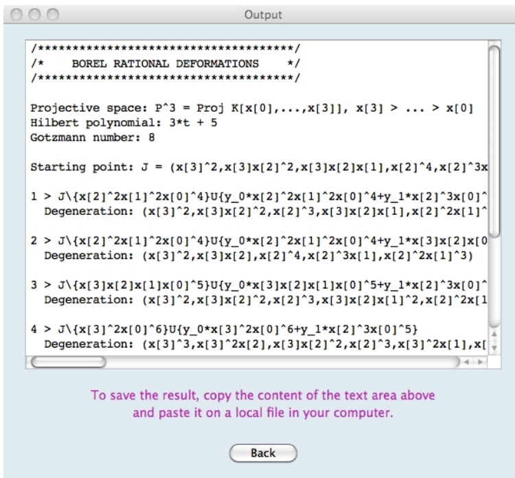
Figure B.6: The output window of the applet Borel Rational Deformations.
