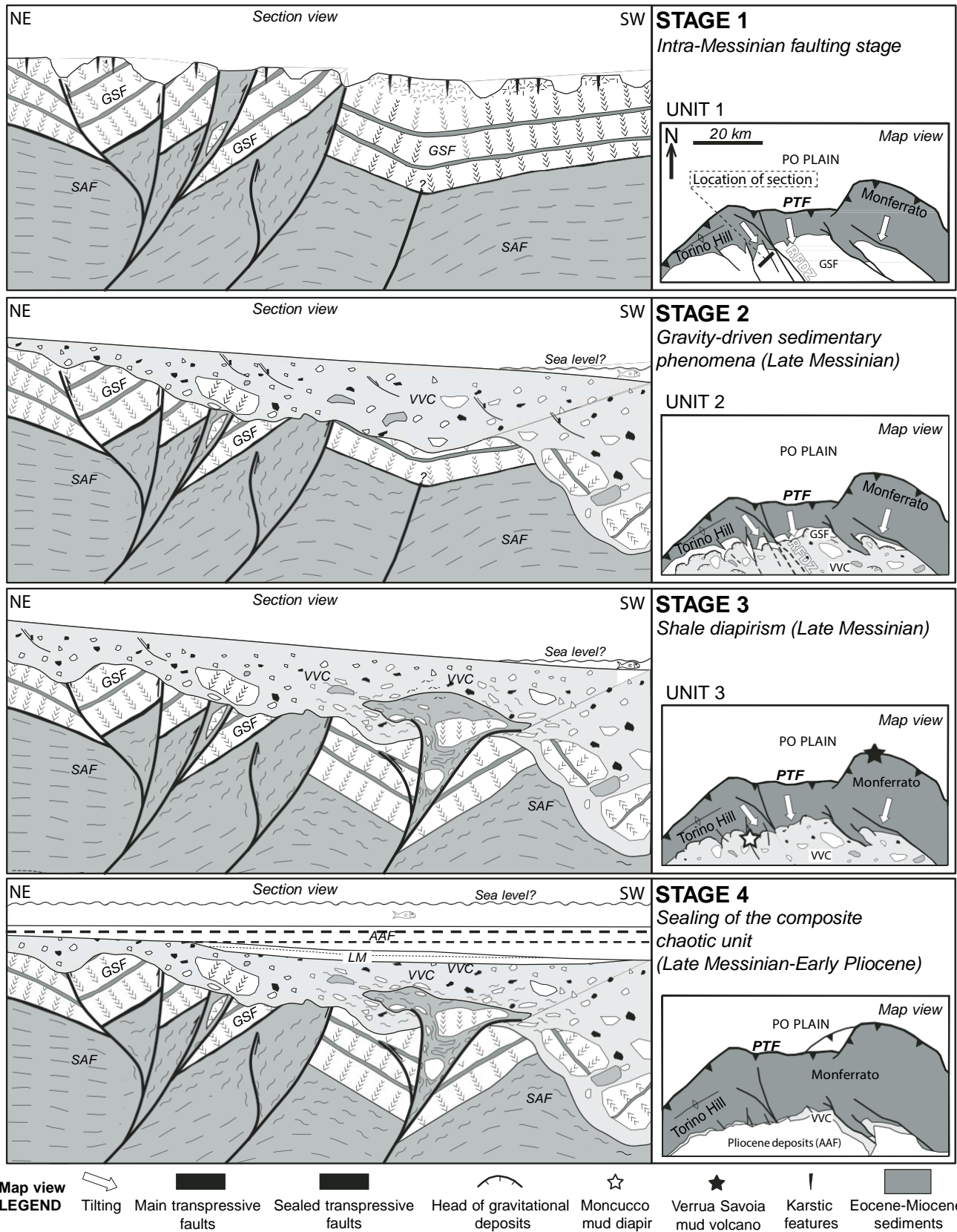
Figure 9. Multistage evolution of the Messinian composite chaotic unit. SAF—Sant’Agata Fossili marls; GSF—Gessoso Solfifera Formation; VVC—Valle Versa chaotic complex; LM—Lago Mare marls; AAF—Argille Azzurre Formation; PTF—Padane thrust front; RFDZ—Rio Freddo deformation zone. For more details, see the text.
