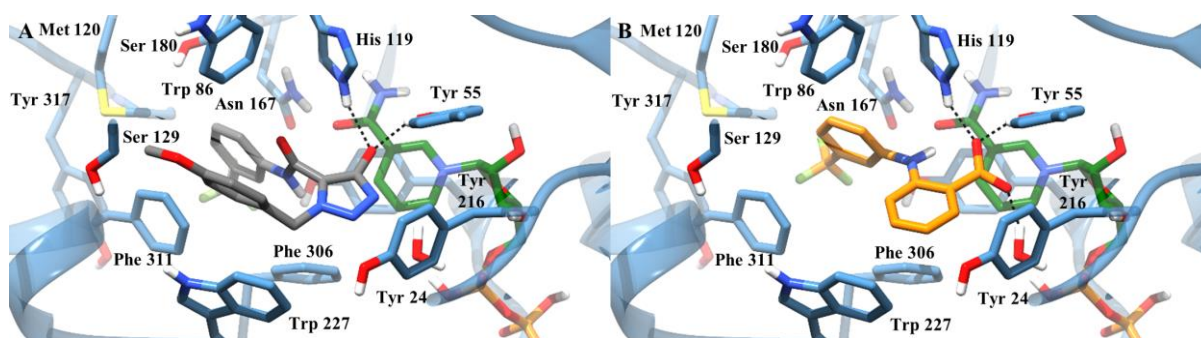
Figure 5. Compound 8 (grey, A) and FLU (orange, B) docked in the AKR1C3 binding site. NADP + is coloured in green.
