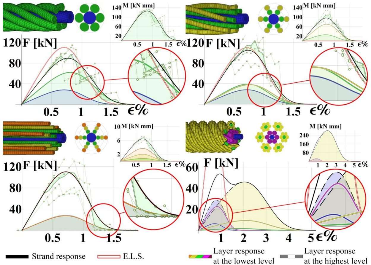
Figure 5. Analytical and FE models with results (axial force F and torque M versus elongation \varepsilon ) for a simple straight strand 6X1 ( top-left ), a multilayered straight strand 6X6X1 ( top-right ), a multilayered straight strand 6X6X6X1 ( bottom-left ) and a hierarchical strand 6X1-6X1 ( bottom-right ). Geometrical parameters are reported in Table 2, while wire material parameters are those already indicated for Figure 4. Results for a tensile test are illustrated for the case in which twisting is not permitted. The black lines refer to the overall strand response, the coloured lines refer to the response of the single layer at the lowest hierarchical level in the strand (illustrated using the corresponding colour in the graphics above), the grey dashed lines denote the single layer response at the highest hierarchical level in the strand (shaded with the blue, green, yellow and red colour in case of core, 1 st , 2 nd and 3 rd external layer respectively), while the red thick lines indicate the results obtained from ELS hypothesis, here obtained as special case of the proposed theory as in Eq. (32). Note that ELS does not capture the coupling between torsion and elongation.
