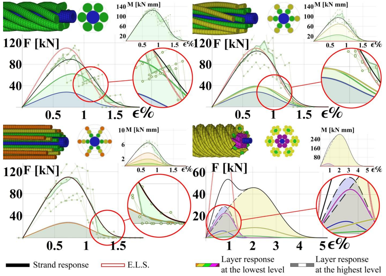
Figure 5. Analytical and FE models with results (axial force F and torque M versus elongation \epsilon ) for a simple straight strand 6X1 ( top-left ), a multilayered straight strand 6X6X1 ( top-right ), a multilayered straight strand 6X6X6X1 ( bottom-left ) and a hierarchical strand 6X1-6X1 ( bottom-right ). Geometrical parameters are reported in Table 2, while wire material parameters are those already indicated for Figure 4. Results for a tensile test are illustrated for the case in which twisting is not permitted. The black lines refer to the overall strand response, the coloured lines refer to the response of the single layer at the lowest hierarchical level in the strand (illustrated using the corresponding colour in the graphics above), the grey dashed lines denote the single layer response at the highest hierarchical level in the strand (shaded with the blue, green, yellow and red colour in case of core, 1 st , 2 nd and 3 rd external layer respectively), while the red thick lines indicate the results obtained from ELS hypothesis, here obtained as special case of the proposed theory as in Eq. (32). Note that ELS does not capture the coupling between torsion and elongation.
