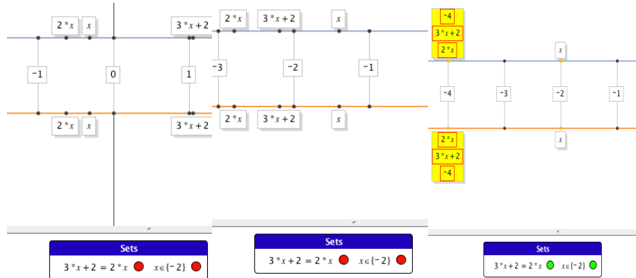
Fig 3a. By dragging x along the line, it is possible to explore the solution of the equation 3x+2=2x . The truth set of the equation is the value -2 .
