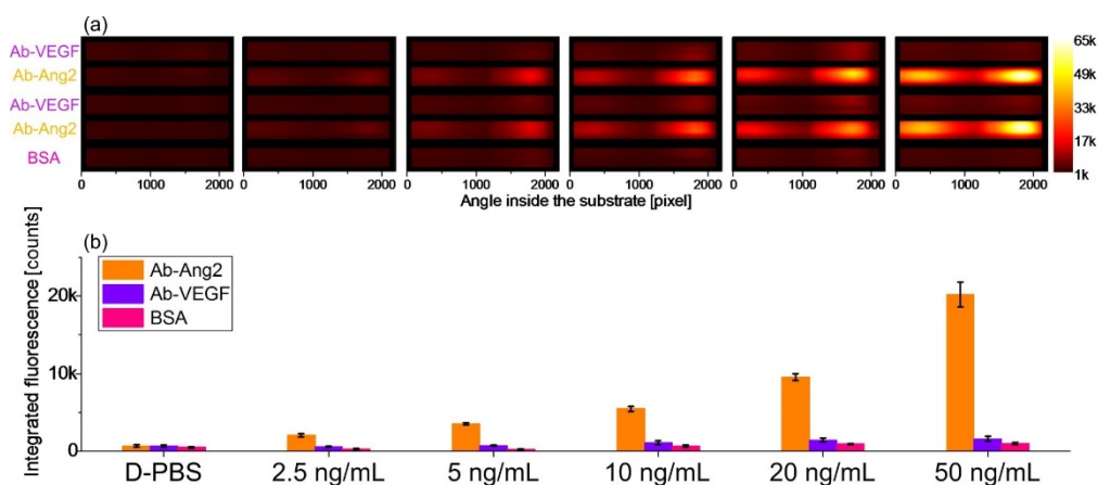
Fig. 5. Fluorescence intensities recorded for the standard Ang2 solutions at different concentrations in D-PBS. (a) Fluorescence intensities recorded by the CCD at the end of the assay. (b) Integrated and averaged intensities for each group of spots on the BSW biochip; the error bars represent the standard deviation associated with the integrated and averaged values.
