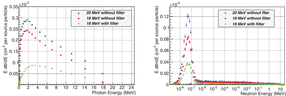
Fig. 2. – The bremsstrahlung photon and the final thermal neutron spectra calculated on a (20 \times 20) \text{ cm}^2 surface with MCNP4B-GN at 50 cm from the target. The lowest curve corresponds to the nominal accelerator configuration; the intermediate one is obtained removing the flattening filter from the Linac head; the highest curve is obtained removing the flattening filter and rising the electron energy up to 20 MeV.
