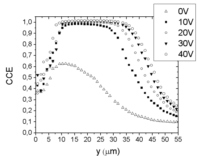
FIG. 3. Charge collection efficiency (CCE) profiles in the depth direction collected at increasing bias voltage (Al electrode on the left).
