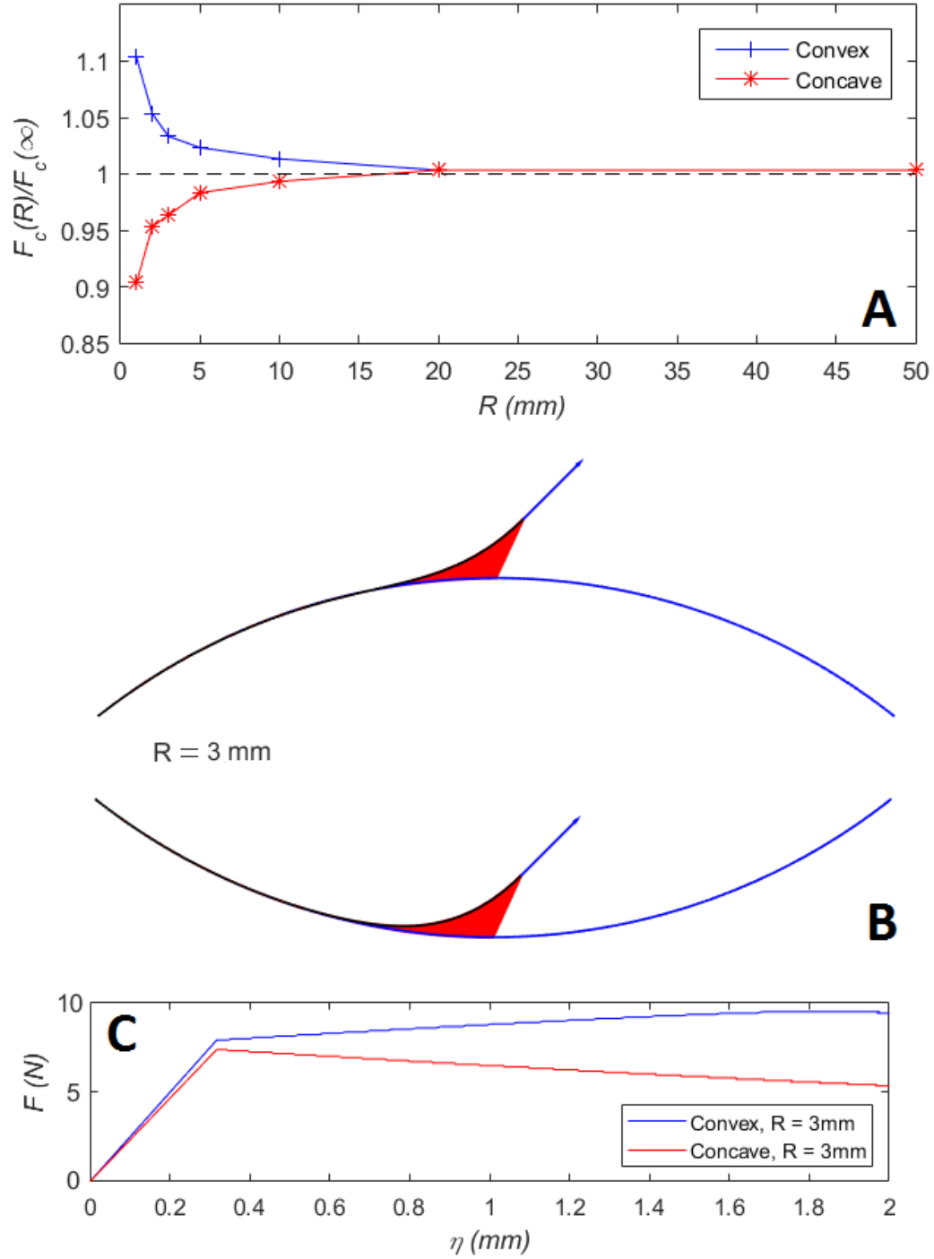
2 Figure 7 : A. Normalized peeling force as a function of the radius of curvature of the substrate for 3 concave and convex surfaces. B. Corresponding deformation states. C. Corresponding force F vs. 4 displacement \eta during peeling test.
