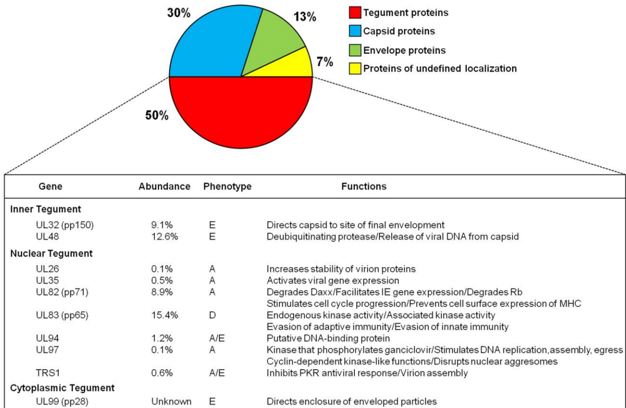
Figure 1 - Genes that encode representative tegument proteins along with commonly accepted protein names are shown. Data on relative abundance were obtained from Varnum et al. (Varnum et al., 2004). Phenotype refers to the ability of virus with a mutation in the indicated gene to replicate in human fibroblasts unless otherwise stated. Phenotypes are listed as augmenting (A), dispensable (D), or essential (E) for virus replication. Functions displays either demonstrated or inferred functions for these proteins.
