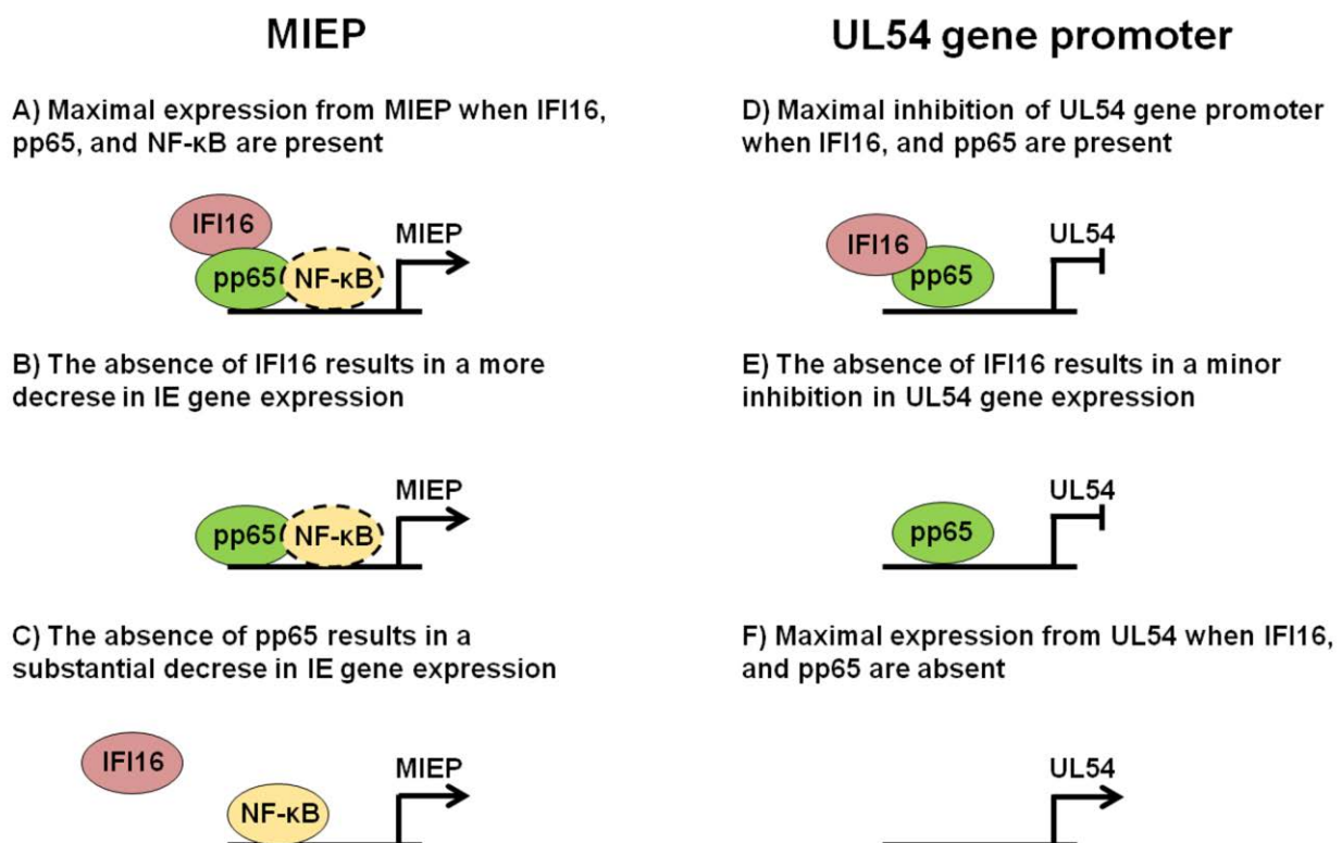
Figure 3 - Interplay between pp65 and IFI16 during HCMV infection. (A) Wild type infection allows maximal activation of the MIEP through efficient recruitment of IFI16 and probably NF- \kappa B (dashed line) by pp65. (B) In the absence of IFI16, pp65 can still drive expression from MIEP, albeit less efficiently, perhaps through either a weaker interaction with or less efficient recruitment of NF- \kappa B. (C) In the absence of pp65, IFI16 and NF- \kappa B may still be capable of interacting at the MIEP, though MIEP expression is decreased indicating the requirement of pp65 for maximal expression. (D) Wild type infection allows maximal inhibition of the UL54 gene promoter through efficient recruitment of IFI16 by pp65. (E) In the absence of IFI16, pp65 can still drive expression from UL54 gene promoter, albeit less efficiently. (F) In the absence of pp65, and IFI16 may still be capable of interacting at the UL54 gene promoter, though UL54 gene promoter inhibition is absent indicating the requirement of pp65 for maximal inhibition.
