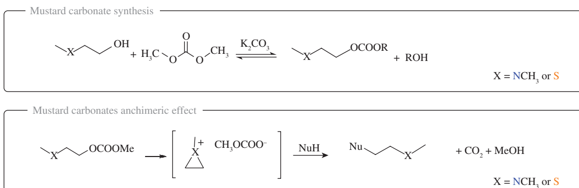
Fig. 2: Molecular structure, synthesis and reactivity of mustard carbonates.
