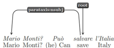
Figure 4: Examples of newly-introduced label extensions for paratactic structures in PoSTWTITA-UD.
