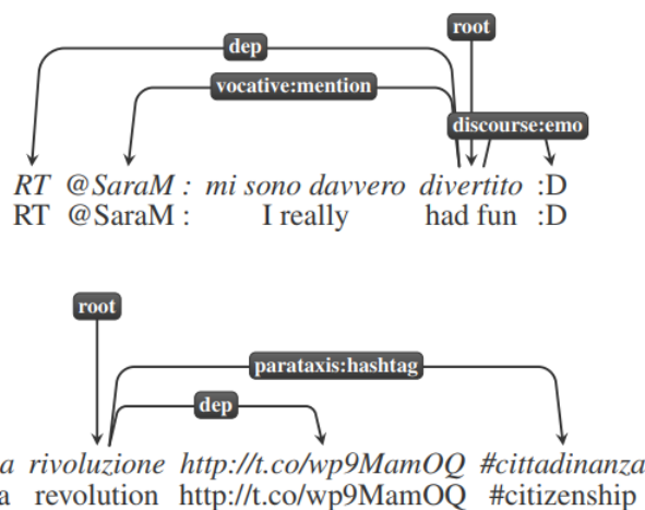
Figure 2: Examples of relations for meta-language tokens in PoSTWTITA-UD.
