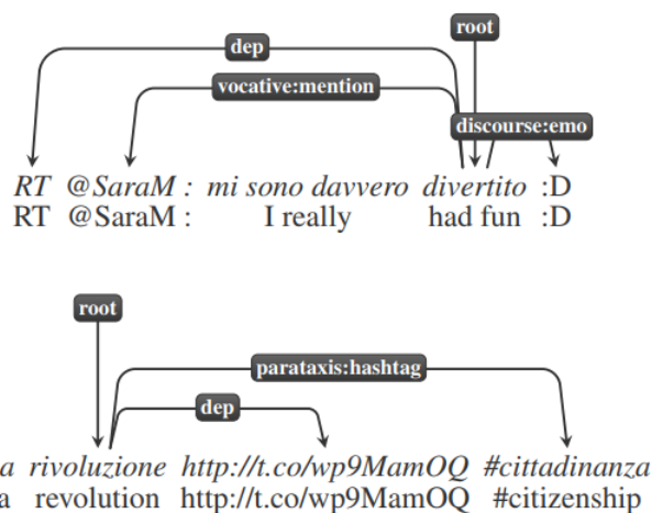
Figure 2: Examples of relations for meta-language tokens in PoSTWITA-UD.
