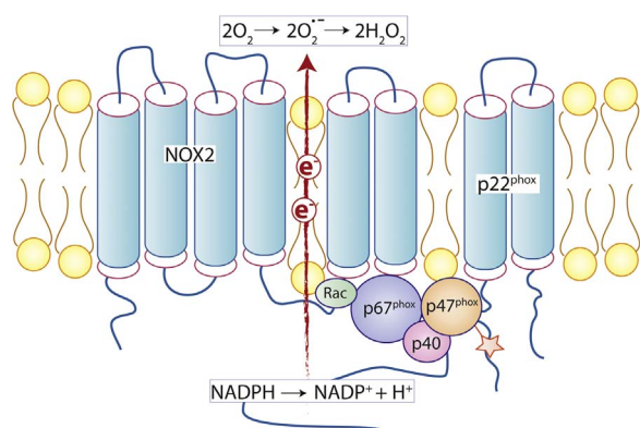
Fig. 1. Schematic structure of the phagocyte NADPH oxidase NOX2. The catalytic complex is formed by the membrane association of NOX2 and p22 phox . Upon activation a cytosolic complex is formed and translocates to the membrane in order to form an active O_2^{\cdot -} -generating enzymatic system.
