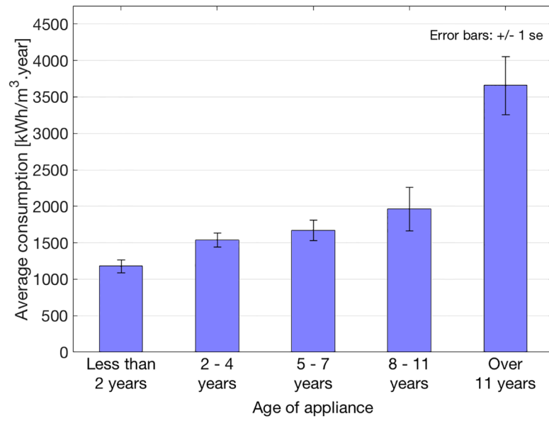
Fig. 15. Average specific energy consumption [kWh/m³·year] by appliance age.
