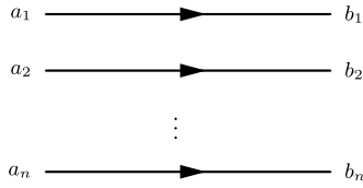
Fig. 3. The diagram representing the tree-level correlator (3.21).
