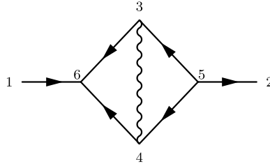
Fig. 9. Irreducible two-loop box diagram contributing to W_2 .
