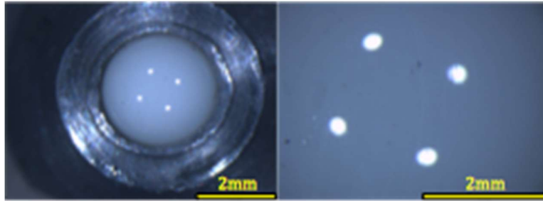
Figure 12. \text{Al}_2\text{O}_3 ball head after the wear test at different magnifications.
