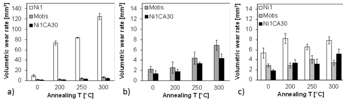
Figure 5. from left to right: calculated wear values for Ni1, Motis, and Ni1CA30 in dry conditions (a), and detailed magnification for Motis and Ni1CA30 (b); and wear values for Ni1, Motis, and Ni1CA30 in lubricated conditions (bovine serum, c).
