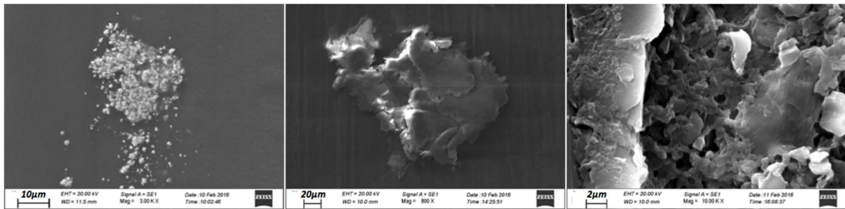
Figure 13. typical debris observed for each tested condition for unfilled ( \text{Ni}_1 , left) and CFR PEEK ( \text{Ni}_1\text{CA}_{30} , middle and right). No sign of fiber pull out could be observed.
