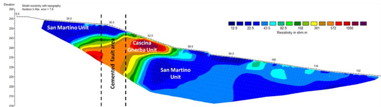
Fig. 4 - Resistivity distribution along the Cascina Volpiano geophysical survey line, with reported geological interpretation.
