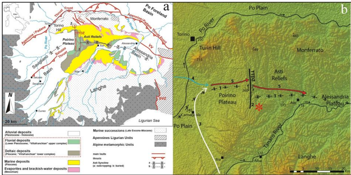
Fig. 1 - a) Simplified geological map of the Piedmont hilly region with the location of the TTDZ; b) Aster Global DEM (NASA-MITI, Dec. 2009) showing the scarp between the Poirino Plateau and the Asti Reliefs. (1) Asti Syncline axis; (2) T. Traversola Deformation Zone (TTDZ); Upper Pleistocene ancient course of rivers: (3) Tanaro, (4) Po, (5) Po and Tanaro. The asterisk indicates the location of Fig. 2 (from Gattiglio et al., 2015).
