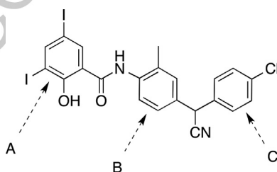
f0055 Fig. 10 The closantel structure (the three rings have been indicated referring to Gloeckner et al. 55 ).
