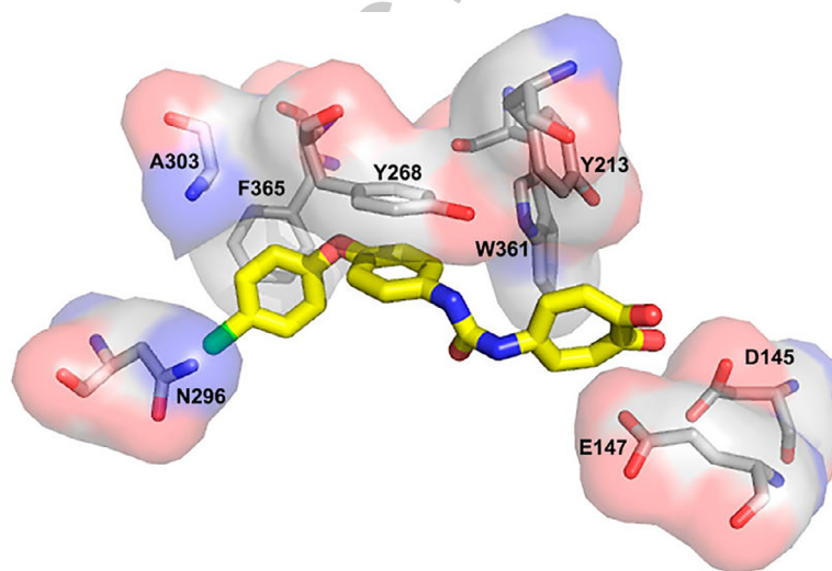
f0070 Fig. 13 Lowest energy pose of compound 3a from Gooyit et al., 61 docked into OvCHT1 (IC 50 0.84 ± 0.01) using the program AutoDock Vina. Color scheme: oxygens in red, nitrogens in blue, carbons in yellow (compound 3a ) or gray (OvCHT1).
