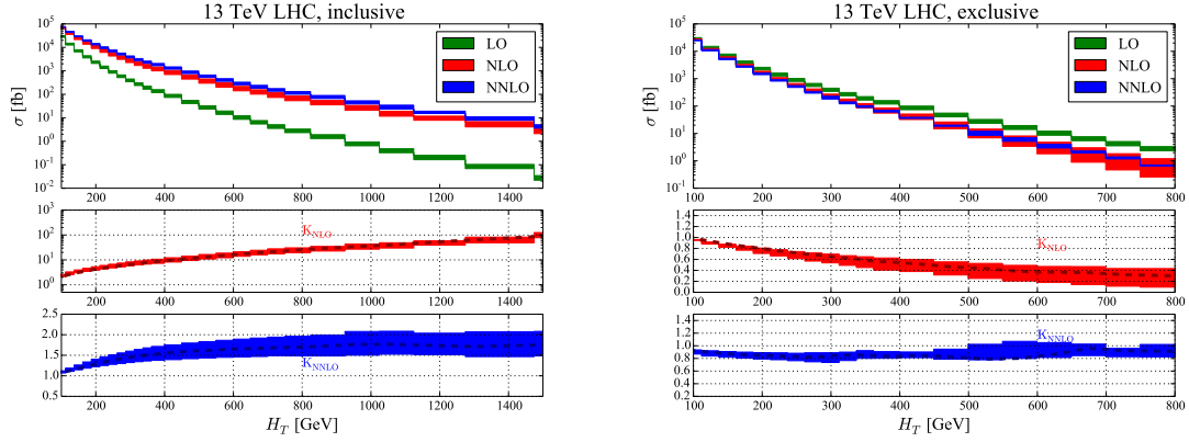
Figure 7. Comparison of the LO, NLO and NNLO H_T distribution for inclusive and exclusive W+1 jet production and the behaviour of the NLO and NNLO K-factors (below). Figure taken from Ref. [25].
