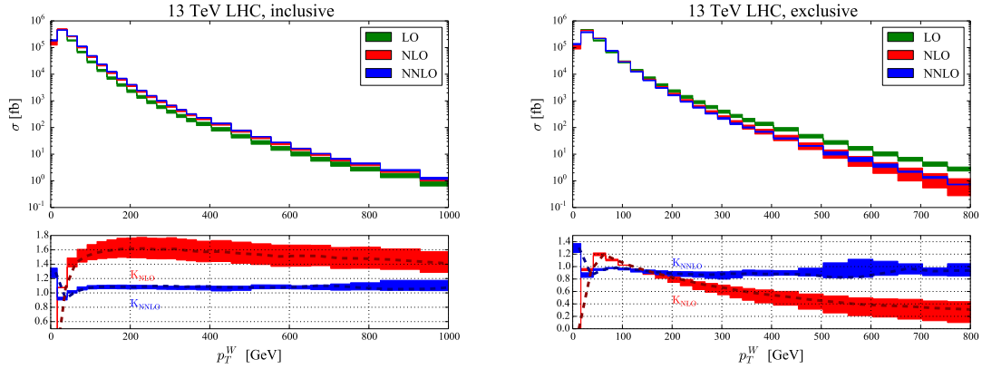
Figure 6. Comparison of the LO, NLO and NNLO p_T^W distribution for inclusive and exclusive W+1 jet production and the behaviour of the NLO and NNLO K-factors (below). Figure taken from Ref. [25].
