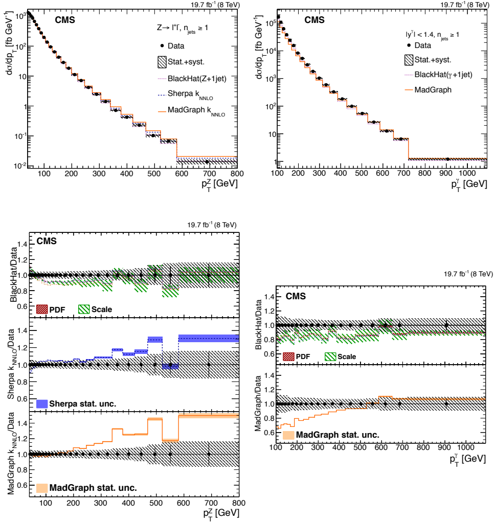
Figure 2. Differential cross section of Z+jets production as a function of p_T^Z and \gamma +jets production as a function of p_T^\gamma for the detector corrected CMS data compared to several theoretical predictions. Figures taken from Ref. [15].
