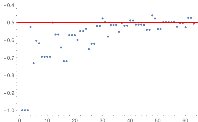
FIGURE 2. The first 64 values of \frac{\log \mathbf{m}_N}{\log L_N} , where L_N = \text{lcm}\{1, \dots, N\} = e^{N+o(N)} , plotted against the constant line -\frac{1}{2} . Les premières 64 valeurs de \frac{\log \mathbf{m}_N}{\log L_N} , où L_N = \text{lcm}\{1, \dots, N\} = e^{N+o(N)} , en comparaison avec la constante -\frac{1}{2} .
