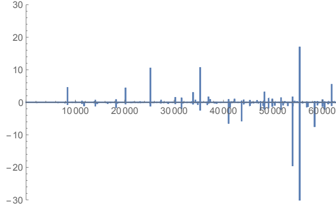
FIGURE 3. Plot of \varrho_N(x)/x for N = 40 and x \in [0, N^3] . Graphe de \varrho_N(x)/x pour N = 40 et x \in [0, N^3] .
