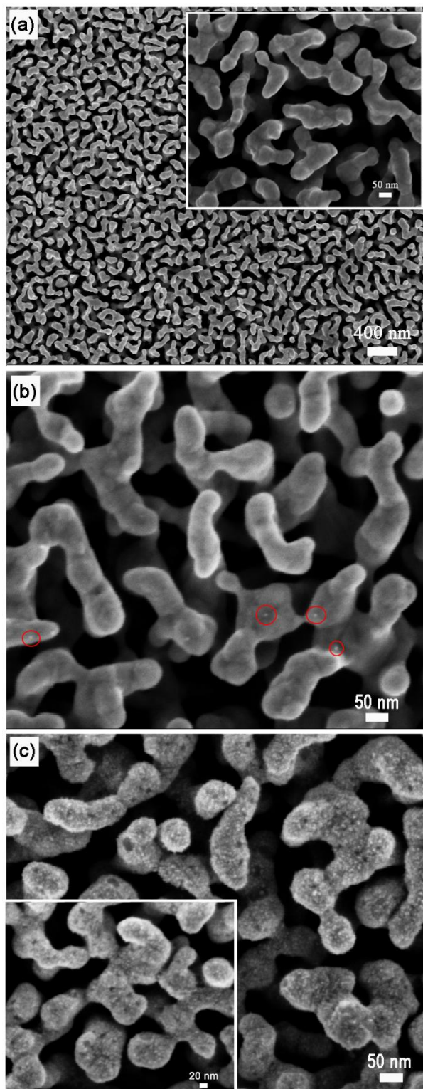
Figure 1. SEM images of (a) the Au 20 Cu 48 Ag 7 Pd 5 Si 20 (at.%) ribbon after chemical de-alloying in 10 M HNO 3 + 0.5 M HF at 70 °C for 4 hours. Samples Pt deposited on nanoporous gold in 0.7 mM H 2 PtCl 6 and 0.5 M H 2 SO 4 with scan rate of 20 mV/s for (b) 5 cycles and (c) 30 cycles. Insets show the corresponding high magnification images.
