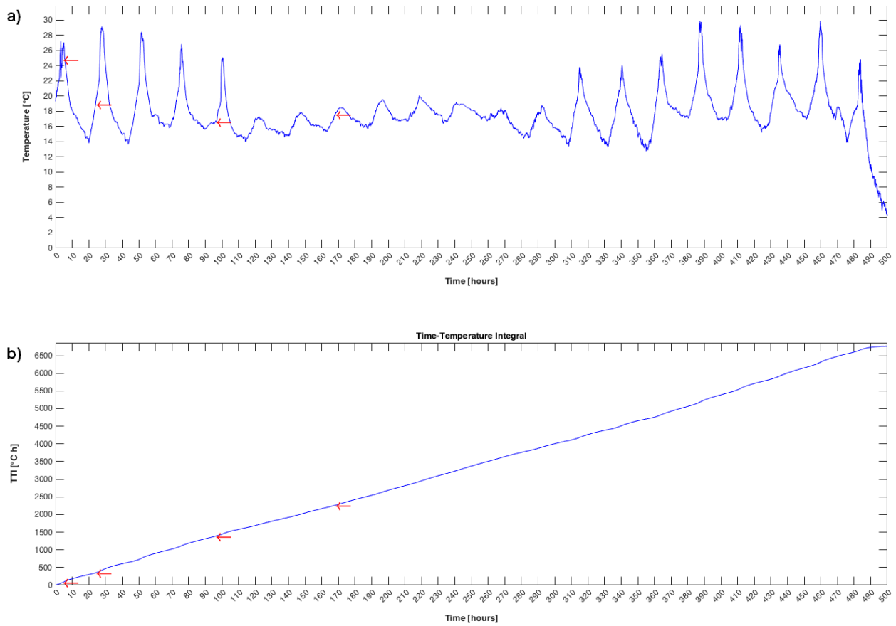
Figure S1. Temperature (a) and Time-Temperature Integral (TTI, b) registered during the postharvest storage/withering of grapes treated with electrolyzed water. Sampling times are marked with a red arrow.
