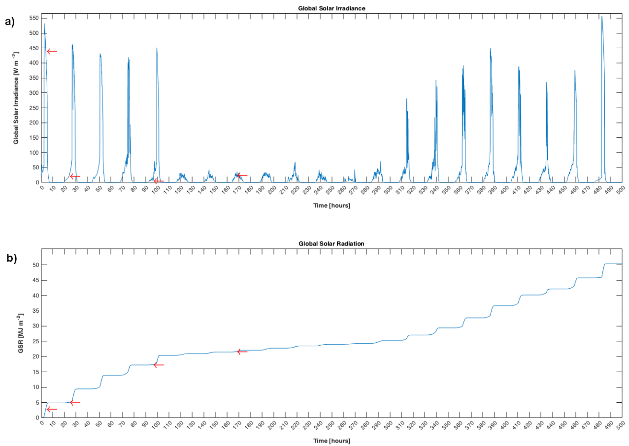
Figure S2. Global Solar Irradiance (a) and Global Solar Radiation (GSR, b) registered during the postharvest storage/withering of grapes treated with electrolyzed water. Sampling times are marked with a red arrow.
