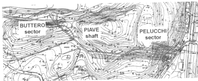
Figure 3 plan of the Olgiate Molgora mine sectors
