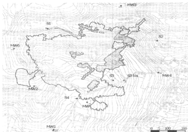
Figure 2 Sketch of the quarry area with the location of sludge storages and drillholes(MW and S series).
