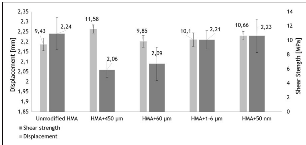
Figure 6. Average shear strength and maximum displacement.
