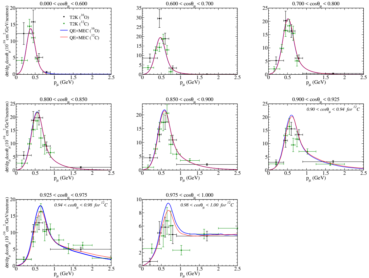
FIG. 5: (Color online) Similar to Fig. 3, but now including also the results corresponding to the T2K- \nu_\mu CCQE process on ^{12}\text{C} . The data are from [1, 46]
