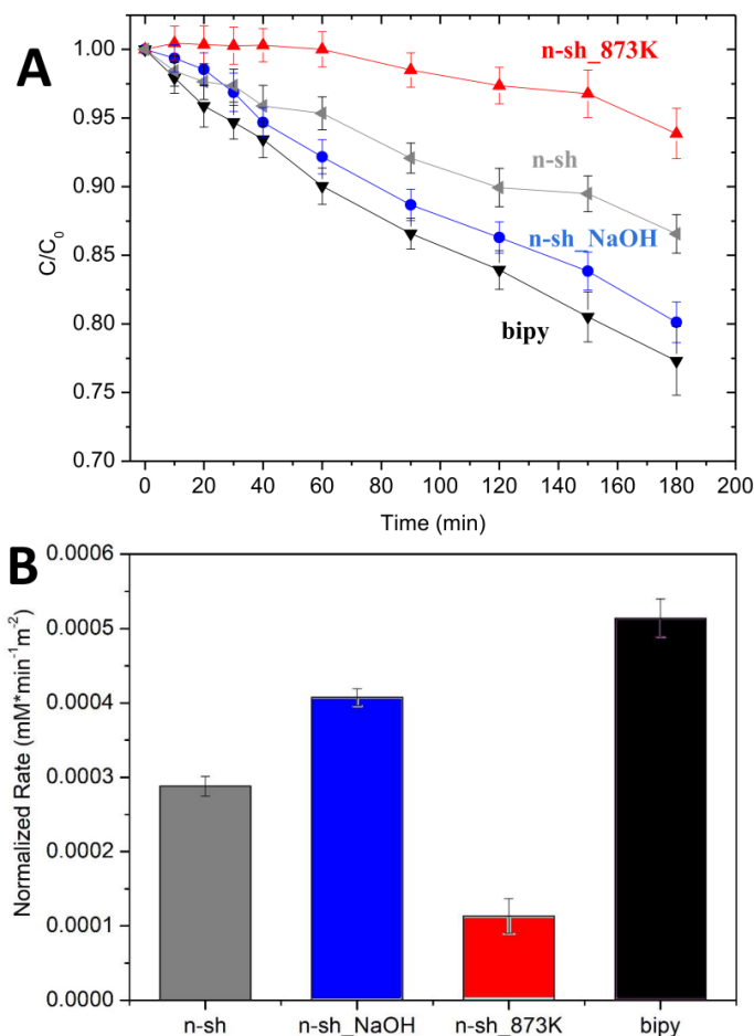
Figure 7. Phenol photodegradation curves (A) and related initial degradation rates, normalized by weight and specific surface area, (B) obtained using the various types of \text{TiO}_2 NPs.
