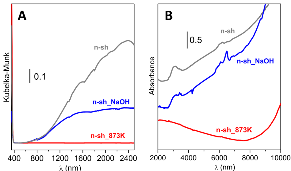
Figure 3. Diffuse reflectance spectra, in the 380-2500 nm range and in Kubelka-Munk units (A), and transmission NIR-MIR spectra, in the 2000-10000 nm range and in absorbance units (B) of TiO 2 n-sh, TiO 2 n-sh_NaOH and TiO 2 n-sh_873K. On the X-axis of panel B, where spectra in the MIR range are shown, wavelength values are reported, instead than conventional wavenumber values, for the sake of consistency with spectra in panel A (being wavelength values commonly used for electronic spectra in the UV-Vis-NIR ranges). Note on the MIR spectrum of TiO 2 n-sh_873K: the apparent decrease in absorbance from 8000 to 2000 nm is the typical effect of decreased scattering of the samples at higher wavelengths, observed when measuring the spectrum in transmission, instead of in diffuse reflectance.
