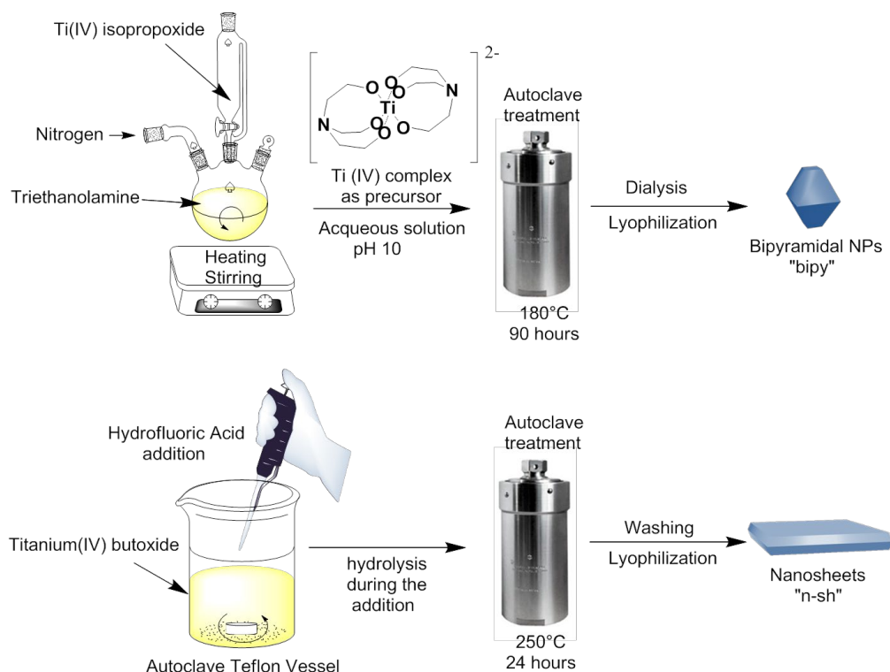
Scheme 1. Synthesis of TiO 2 nano-sheets and TiO 2 bipyramidal nanoparticles.
