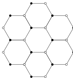
FIGURE 2. A hexagonal groundstate
