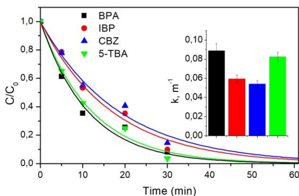
Figure 2. Photo-Fenton-like degradation of CEC mixture (20 \mu\text{M} ) in real wastewater. Conditions: pH 3, \text{H}_2\text{O}_2 1.0 mM, \text{Fe}_3\text{O}_4/0.5\text{HA} 100 \text{mg dm}^{-3} (MPs synthesized with HA solution 0.5%). Inset: first-order kinetic constants of the process.
