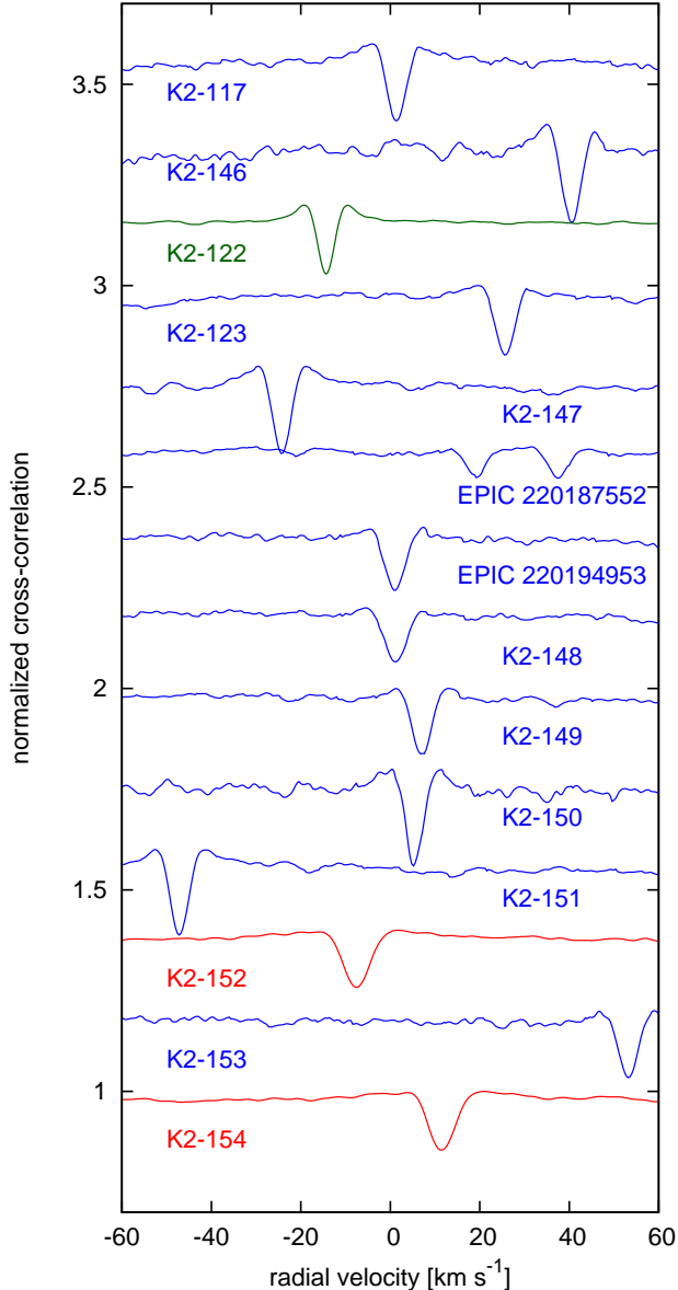
Figure 4. Averaged and normalized cross-correlations between the observed spectra and M2 binary mask. Cross-correlations based on the HDS, HARPS-N, Tull spectra are shown in blue, green, and red, respectively. The Earth’s motion is corrected and RV value is given with respect to the barycenter of the solar system.
