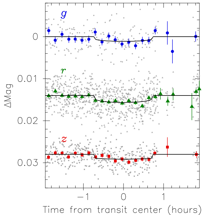
Figure 13. Ground-based transit observation for K2-151 by OAO/MuSCAT (grey dots). The binned flux data for g' -, r' -, and z_s -bands are shown by the blue circles, green triangle, and red squares, respectively. The black solid lines indicate the best-fit transit models for individual bands.
