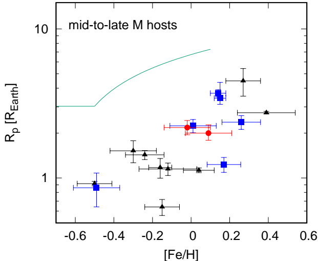
Figure 21. Host stars’ metallicities from spectroscopy vs. radii of the planets around mid-to-late M dwarfs ( T_{\text{eff}} \leq 3500 K). For multi-planet systems, the largest planets are plotted. Symbols are the same as in Figure 18.
