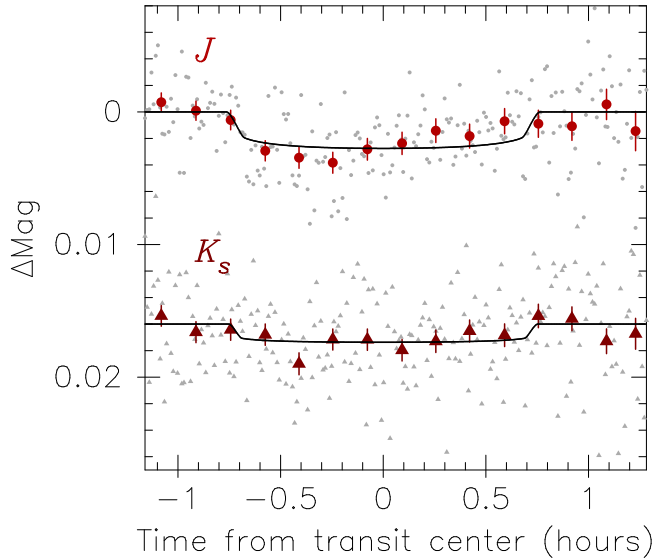
Figure 14. Ground-based transit observation for K2-151 by IRSF/SIRIUS (grey dots). The binned flux data for J -, and K_s -bands are shown by the dark-red circles, brown triangles, respectively. The black solid lines indicate the best-fit transit models for individual bands.
