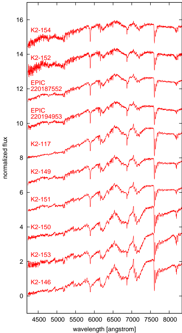
Figure 1. Wavelength-calibrated, normalized optical spectra observed by CAFOS. Later M dwarfs are plotted towards the bottom.
