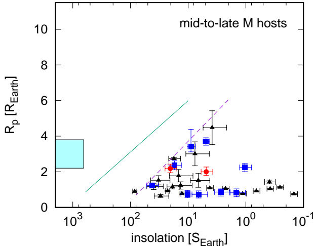
Figure 19. Stellar insolation fluxes vs. radii of planets around mid-to-late M dwarfs ( T_{\text{eff}} \leq 3500 K). Symbols and plot ranges are the same as in Figure 18.
