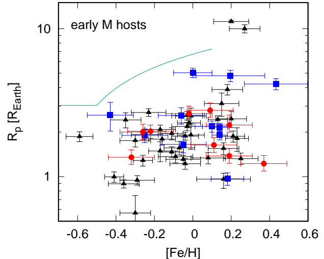
Figure 20. Host stars’ metallicities from spectroscopy vs. radii of the planets around early M dwarfs ( 3500 \text{ K} < T_{\text{eff}} \leq 4000 \text{ K} ). For multi-planet systems, the largest planets are plotted. Symbols are the same as in Figure 18 . Note that contrary to Figures 18 and 19 , the y -scale is logarithmic.
