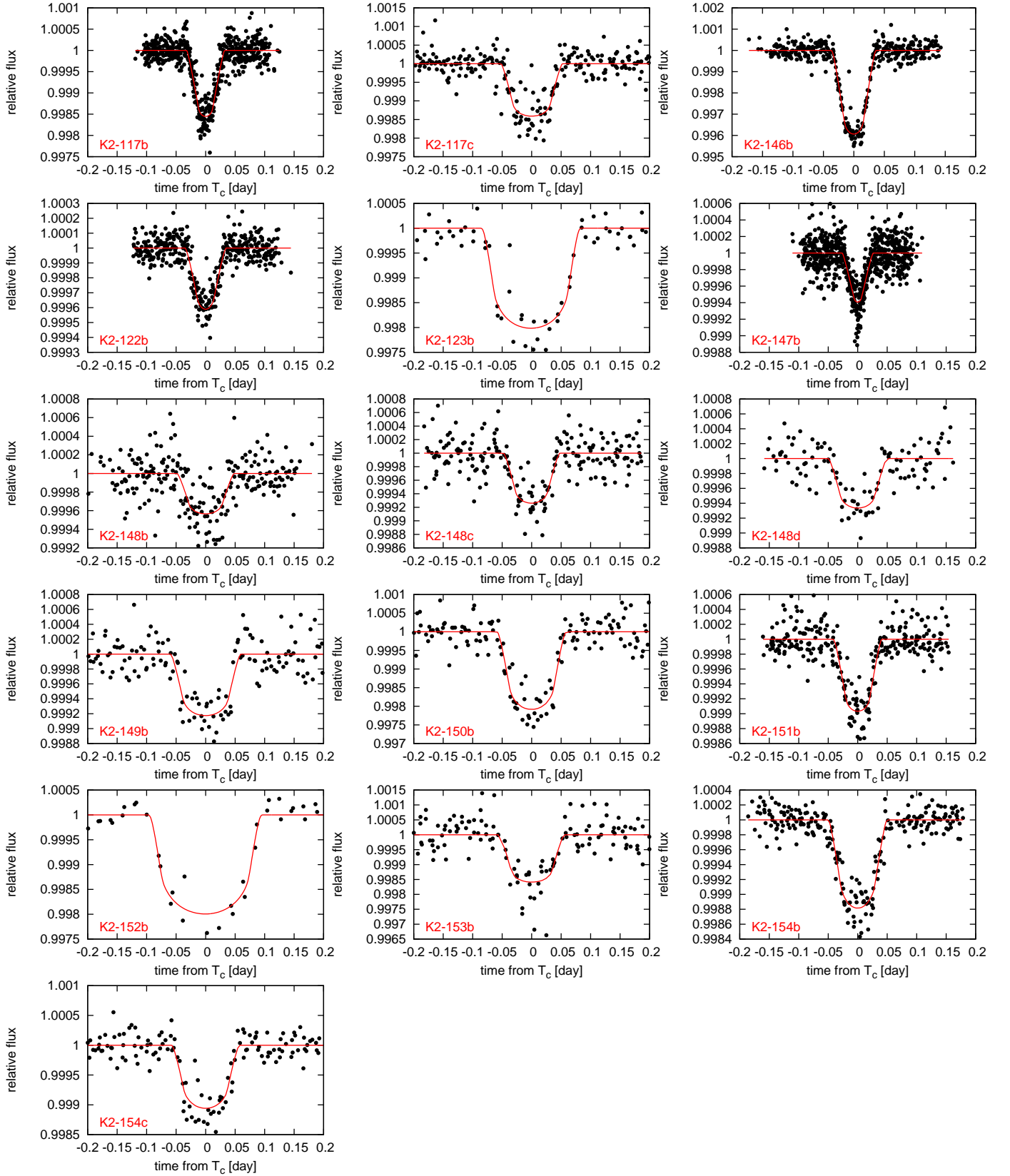
Figure 6. K2 light curves around transits for individual candidates folded by their periods. Possible TTVs are corrected and all the transits are aligned in these light curves. For K2-148, the flux contamination from EPIC 220194953 is taken into account and the dilution factor is corrected. The best-fit transit curves are shown by the red solid lines.
