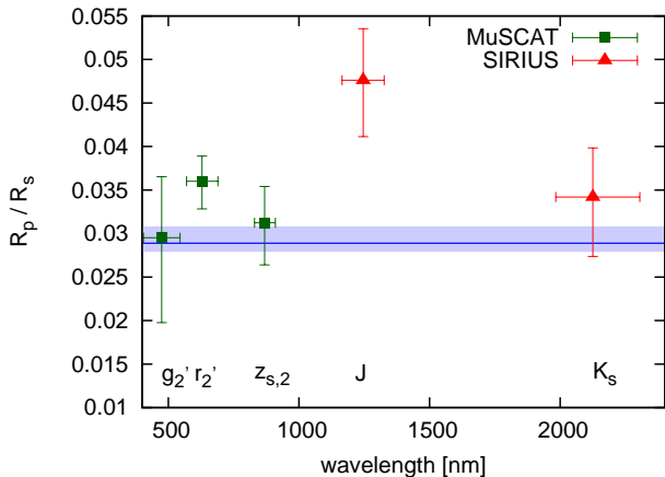
Figure 15. Observed R_p/R_s values of for K2-151b in different bandpasses. The blue horizontal line and its upper and lower shaded areas indicate R_p/R_s and its \pm 1\sigma errors in the K_p band.
