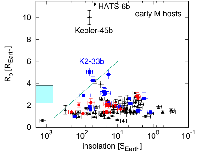
Figure 18. Stellar insolation fluxes vs. radii of planets around early M dwarfs ( 3500 \text{ K} < T_{\text{eff}} \leq 4000 \text{ K} ). Our newly validated planets (red circles), other planets discovered by K2 (blue squares), and planets from the Kepler primary mission and other surveys (black triangles). The cyan rectangle area is the “hot-super-Earth desert” described by Lundkvist et al. (2016) . See the text for the upper boundary of R_p (green solid line).
