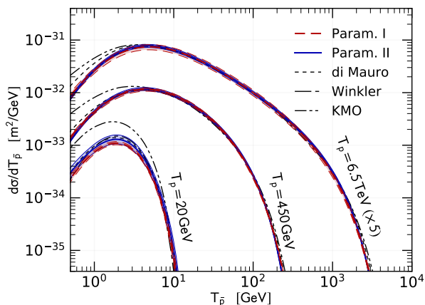
FIG. 4. The differential cross section d\sigma/dT_p(p + p \rightarrow \bar{p} + X) for prompt antiprotons, at the representative proton energies T_p = 20 GeV, 450 GeV and 6.5 TeV. The dashed (solid) line and the red (blue) band are the result of our analysis for Param. I and Param. II. The uncertainty band corresponds to the 2\sigma confidence interval. We report for comparison some literature estimations (see text for details). Tables with the full cross section results are provided in the Supplemental Material to this paper.
