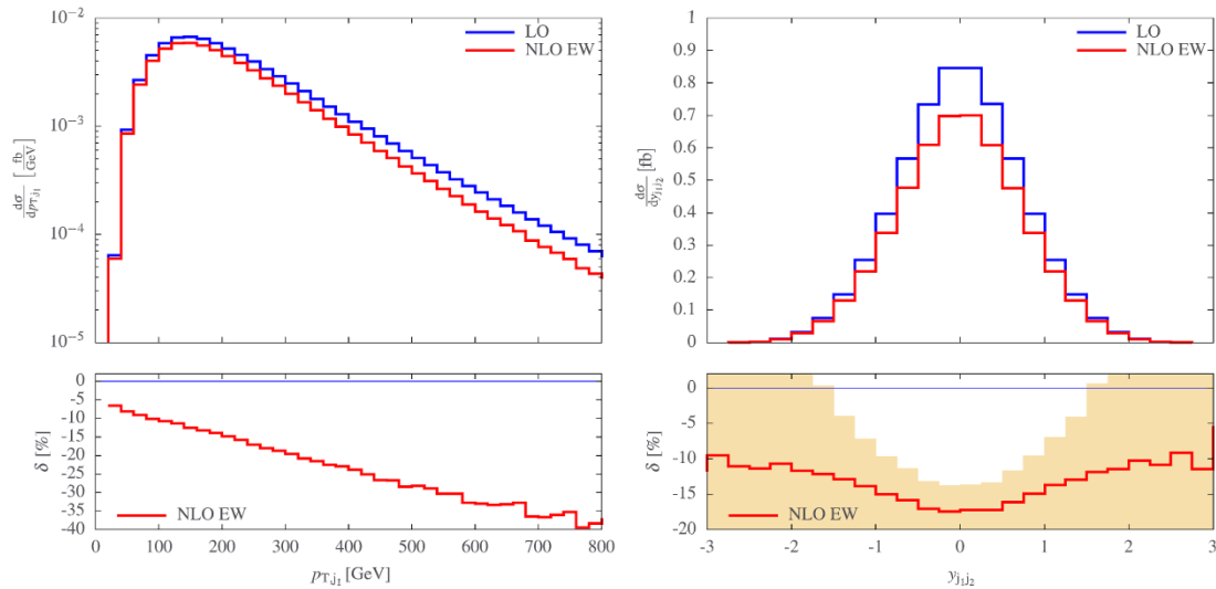
Fig. 2. Differential distributions from Reference [16] for pp \rightarrow \mu^+ \nu_\mu e^+ \nu_e jj including NLO EW corrections (upper panel) and relative NLO EW corrections (lower panel) at \sqrt{s} = 13 TeV. Left plot: Transverse momentum of the most energetic jet. Right plot: Rapidity distribution of the leading jet pair. The yellow band describes the expected statistical experimental uncertainty for a high-luminosity LHC collecting 3000 \text{ fb}^{-1} and represents a relative variation of \pm 1/\sqrt{N_{\text{obs}}} , where N_{\text{obs}} is the number of observed events in each bin. (For interpretation of the references to colour in this figure legend, the reader is referred to the web version of this article.)
