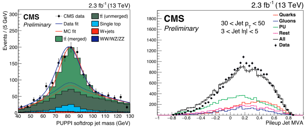
Fig. 11. (Left) Softdrop jet mass of boosted W bosons in data and simulated samples of top pair production in the single lepton plus jets final state. (right) Pileup jet MVA discriminator in data and simulation for jets with |\eta| > 3.0 . The studies have been performed by the CMS collaboration [111].
