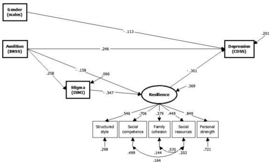
Fig. 1. Diagram of the final SEM. Legend: straight lines indicate direct effects; curved lines indicate correlations; short lines pointing to the dependent variables report explained variance.
